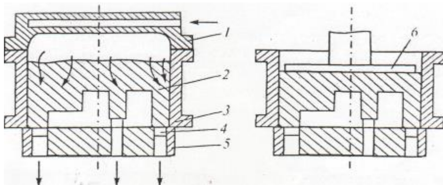
26-rasm. Impuls yordamida aralashmani zichlash:
