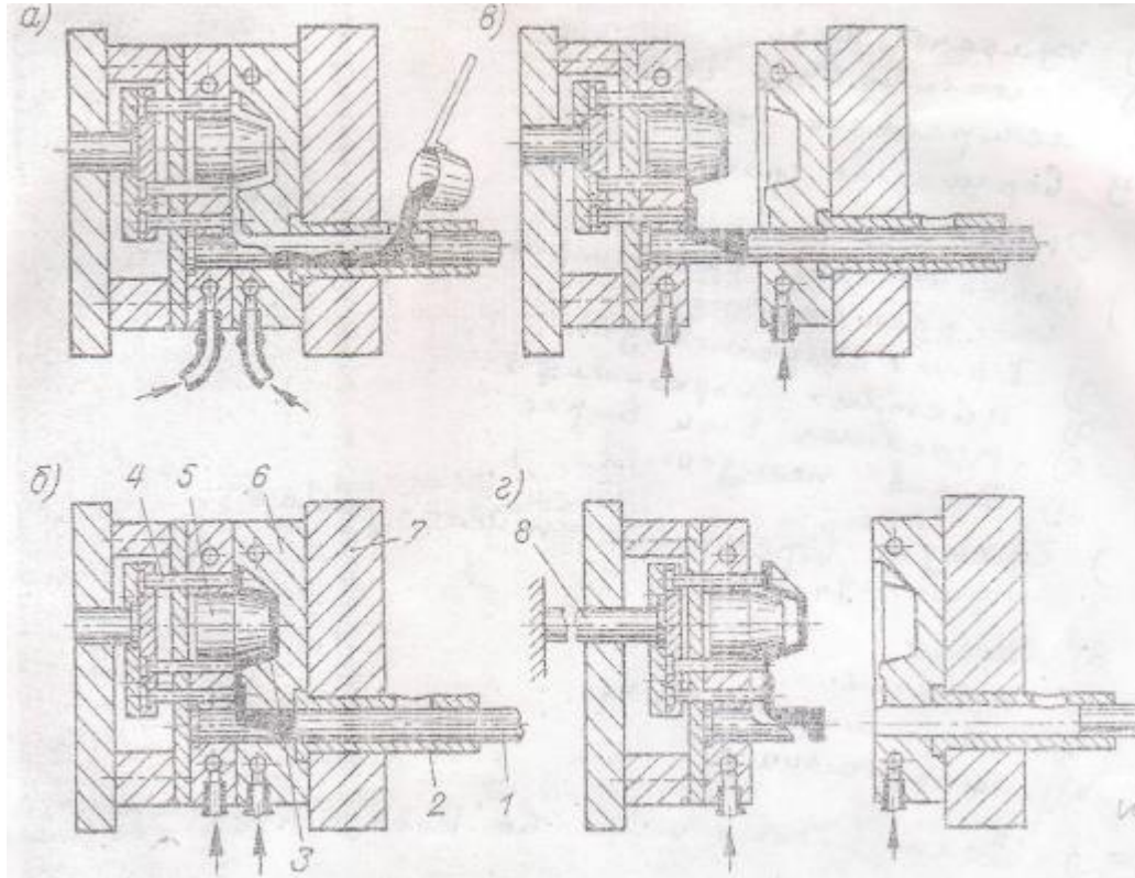
39-rasm. Bosim ostida quyma olishni sxemasi:
