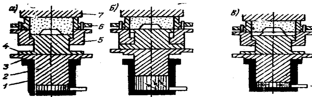
23.1-rasm. Pastdan presslash mashinani ishlash sxemasi
