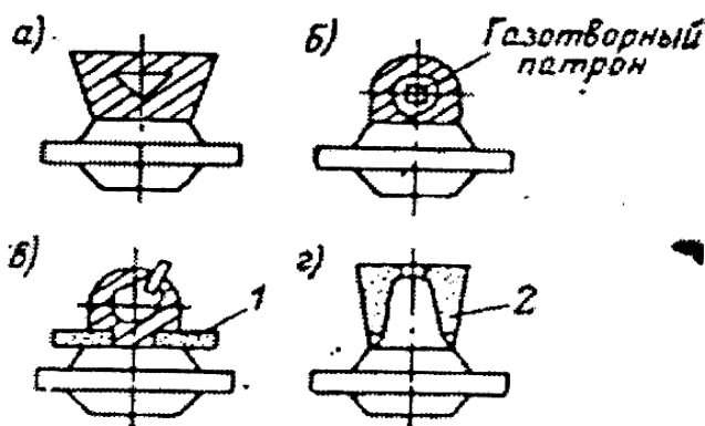
15-rasm. Ustamaning turli qurilmalari
