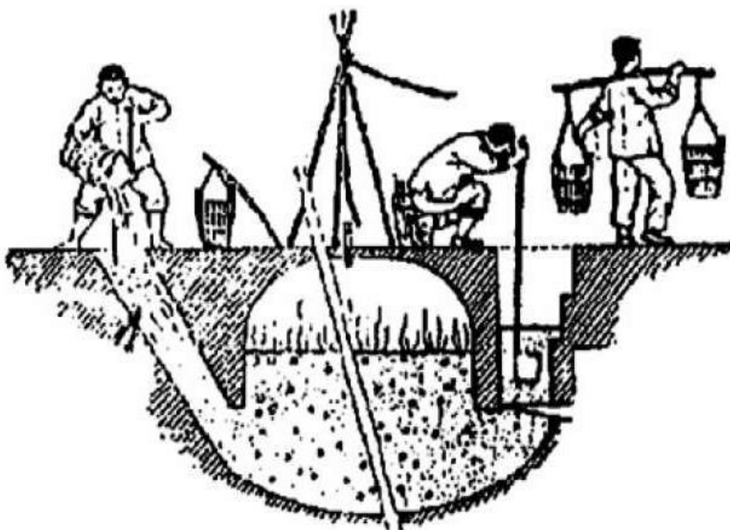
2 – rasm. Biogaz olishning qadimiy Xitoy uskunasi
