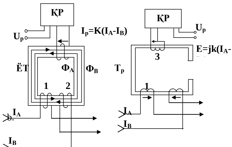
13-rasm. Masofa organlarini ikki faza toki farqiga ulanishi:
