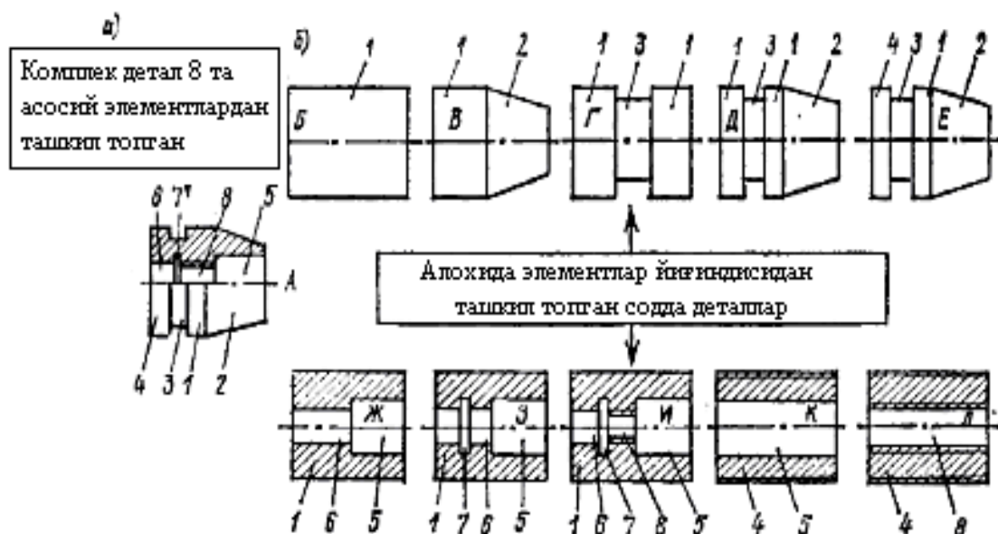
7.7-rasm. Kompleks zagotovkani yaratish:
