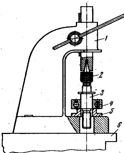
17.6-rasm. Dastaki reykali pressda zoldirli podshipnikni presslab valga kiritish
