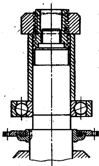
17.5-rasm. Zoldirli podshipnikni valga presslab kirgizish uchun vintli moslama
