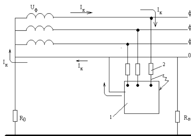
4.3. - rasm. Nolga ulash himoyasini sxemasi
