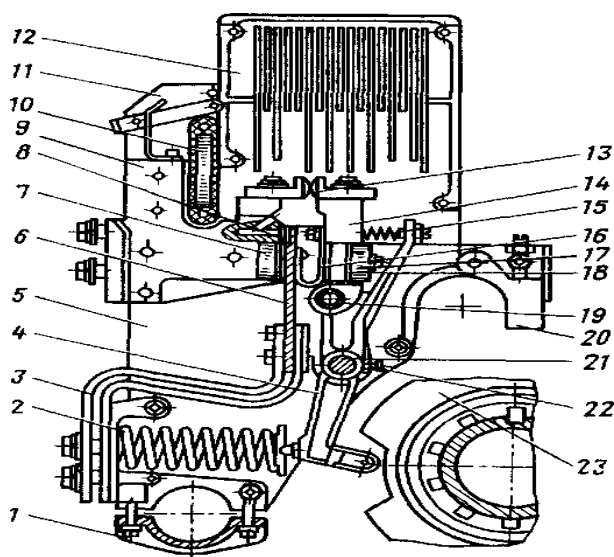
1.1 - rasm. Yoy so`ndirish kamerali mushtumli kontaktor
