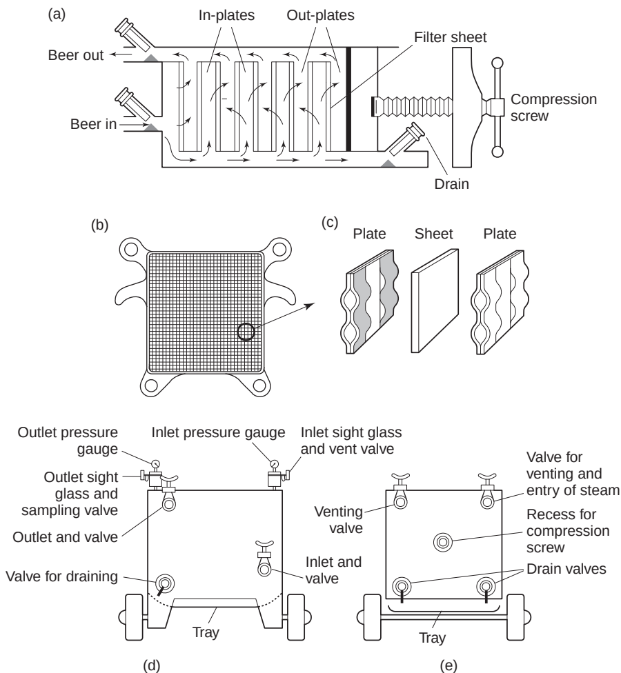
Fig. 15.13 Details of a sheet filter; (a) vertical section, (b) single plate front view, (c) alignment of plates and sheets, (d) control end of machine, (e) compression end of machine (Hough et al. , 1982).
