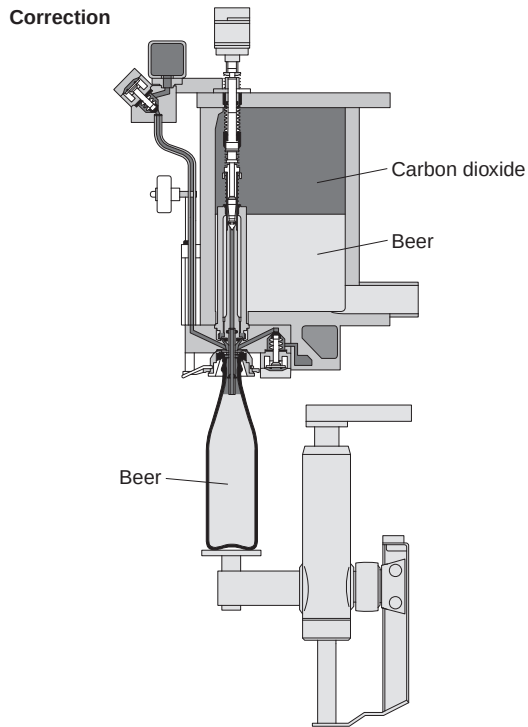
Fig. 21.6 (g) Correction of bottle contents (excess beer displaced back to filling bowl) (by courtesy of Kronen).
