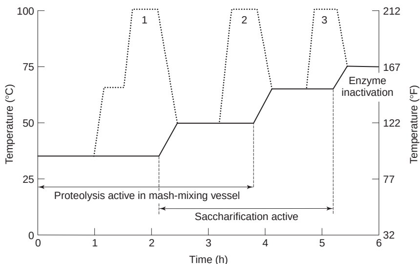
Fig. 4.2 The temperature changes occurring in a typical, traditional triple-decoction mashing programme (after Hind, 1950). —, temperatures in the main mash vessel. .... temperatures in the mash copper during the first, second and third decoctions (1, 2 and 3). About one-third of the mash is used in each decoction. A ‘thick mash’ or a mixed mash may be used. The ‘proteolysis’ and other periods are the oversimplified, traditional names for the divisions of the process. Process duration, about six hours.
