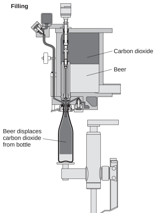
Fig. 21.6 (e) Filling (beer displaces carbon dioxide from bottle) (by courtesy of Krones).
