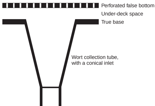
Fig. 6.14 A diagram of a conical entry to a wort collection tube in the base of a lauter tun (after various sources).
