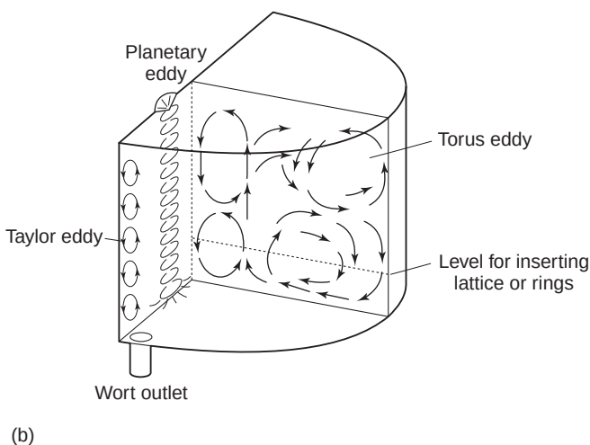
Fig. 10.21 Currents in whirlpool tanks. (a) The ideal flow pattern in a whirlpool. (b) Undesirable eddy currents that can occur and which interfere with trub separation. The most troublesome are the torus eddies, which may be checked by the insertion of a lattice or rings at the level indicated (after Denk, 1991).
