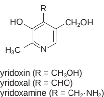
Fig. 4.29 Some water-soluble vitamins and yeast growth factors that occur in wort and ascorbic and dehydroascorbic acids, which occur in green malt.
