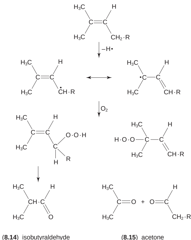
Fig. 8.9 Proposed autooxidation of 3-Methylbut-2-enyl side chains.
