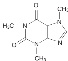
(20.2) Caffeine
