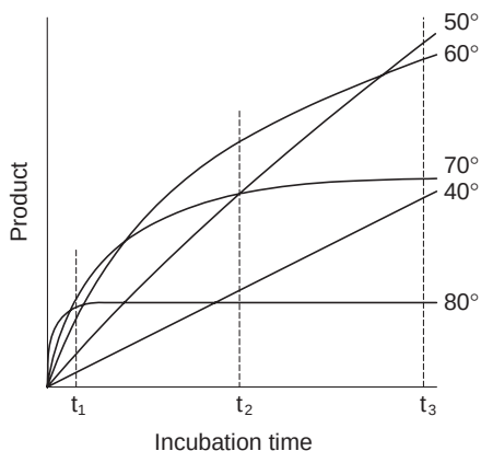
Fig. 4.1 Graphs illustrating the appearance of products in idealized enzyme-catalysed reactions carried out with the initial conditions the same but at different incubation temperatures (°C) (after Dixon and Webb, 1958). As the temperature is increased so the initial reaction rate, at time zero, increases. In the sample, at 40°C the enzyme is stable and so the reaction carries on at a steady rate (substrate is present in excess), and product is formed linearly with time. However, at higher temperatures the enzyme is less stable and so, although the initial reaction rates are more rapid, enzyme is progressively inactivated and the rates of product formation decline. If the maximum amounts of product formed at different times are noted it can be seen that at the shortest time, t_1 , the 'optimum' is at 70°C, at t_2 it is at 60°C while at the longest time, t_3 , it is at 50°C.
