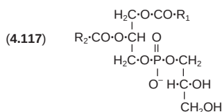
Phosphatidylglycerol
