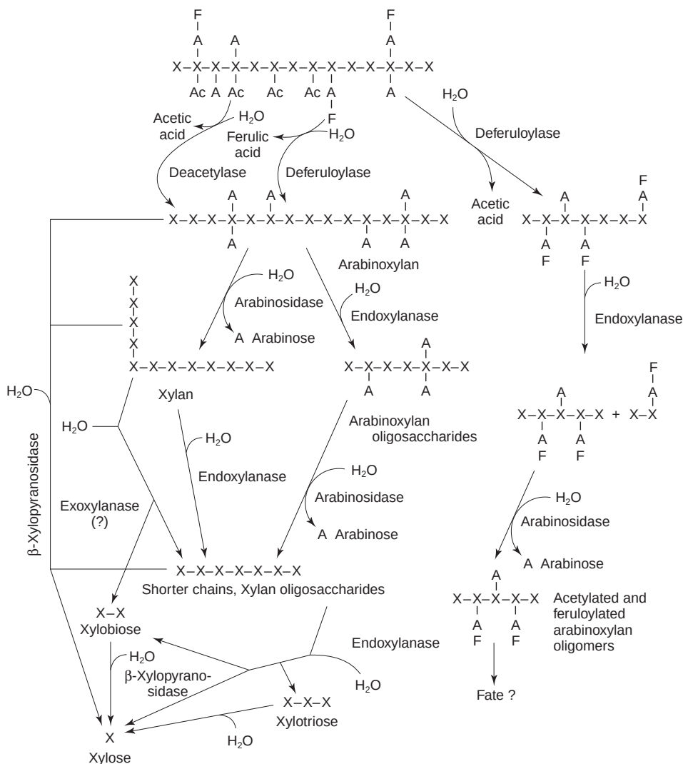
Fig. 4.24 A scheme of the activities of the enzymes believed to be involved in the hydrolytic breakdown of the grain pentosans during malting (Briggs, 1998). X, β-D-xylopyranose residues (4.10) linked (1, 4) in chains. A, α-L-arabinofuranose residues (4.11) Ac and F, acetyl and feruloyl substituents, acetic acid and ferulic acid (4.131) attached to the polysaccharide through ester links.
