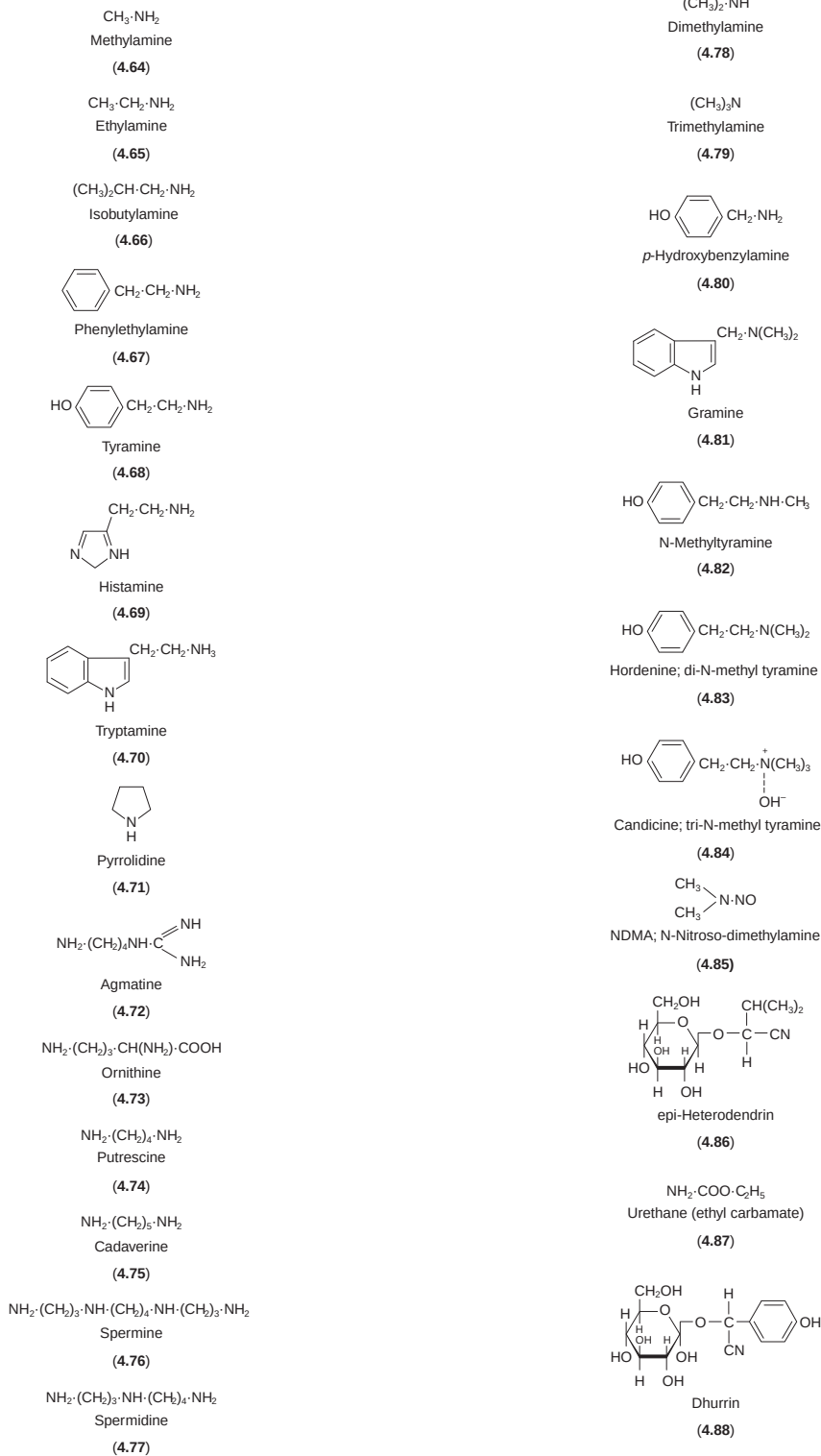
Fig. 4.28 Some amines and other nitrogenous substances found in wort.
