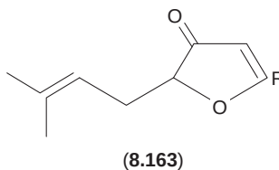
Fig. 8.24 Oxygen heterocyclic compounds in hop oil.
