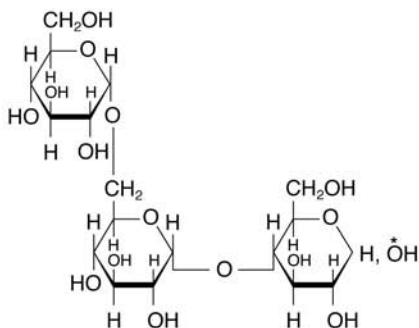
Panose (4- \alpha -isomaltosyl-D-glucose)
