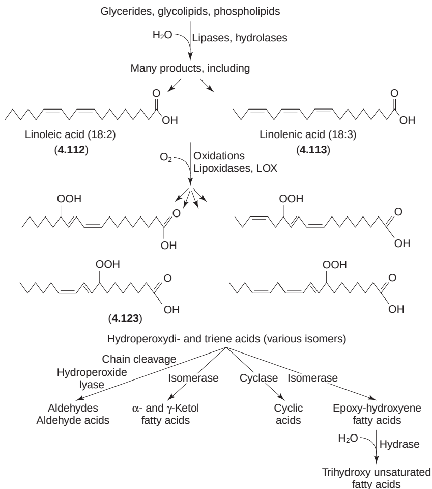
Fig. 4.32 Possible stages in the oxidative breakdown of the major unsaturated fatty acids during mashing (after Briggs, 1978; Gardner, 1988). The number of possible products is very large indeed. It is thought that the unsaturated trihydroxy-fatty acids are the precursors of staling flavour compounds in beers.
