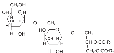
Digalactosyl diglyceride
