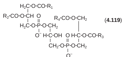
Diphosphatidylglycerol (cardiolipin)
