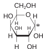
Galactose; \alpha -D-galactopyranose
