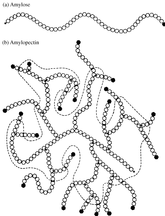
Fig. 4.17 Idealized diagrams of (a) amylose and (b) amylopectin. The chains of D-glucopyranose residues (hexagons) are joined by \alpha -(1, 4)-links in the amylose and the short chains of the amylopectin which are joined together through \alpha -(1, 6)-links, which create branch points, in the amylopectin. The reducing chain ends are marked with an asterisk, while the non-reducing chain ends are indicated with solid hexagons. While the straight chained amylose molecule has only one reducing group and one non-reducing chain end, the highly branched amylopectin has one reducing group but numerous non-reducing chain ends per molecule. The dashed line around the amylopectin indicates the approximate limit of the \beta -limit dextrin remaining after the molecule has been attacked by pure \beta -amylase. The shortened branches, of two or three glucose residues, are readily hydrolysed by limit dextrinase or pullulanase to release maltose or maltotriose. The debranched dextrin can be degraded further by \beta -amylase.
