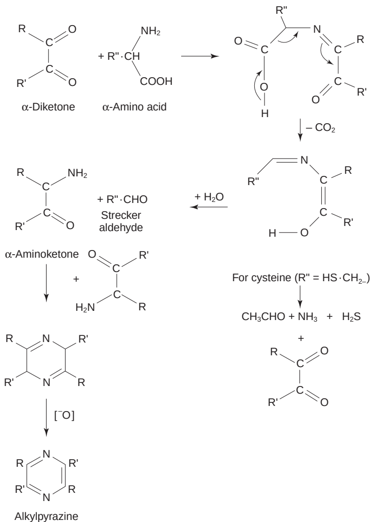
Fig. 9.4 Strecker reaction of \alpha -amino acids and formation of alkylpyrazines.
