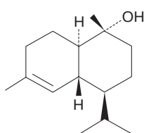
(8.124) α-Cadinol
