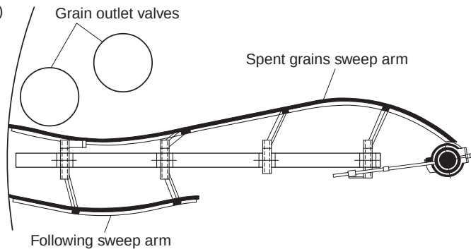
Fig. 6.16 (a) A lauter tun with the grain discharge plough bar in the raised (rest) and lowered (graining-out) working positions (after Barnes, 2000). (b) A plan view of another pattern of grain plough with a trailing, second sweep arm (after Herrmann et al. , 1990).
