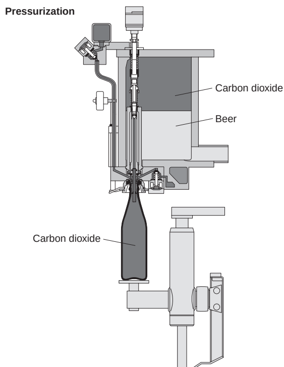
Fig. 21.6 (d) Pressurization (carbon dioxide in bottle) (by courtesy of Krones).
