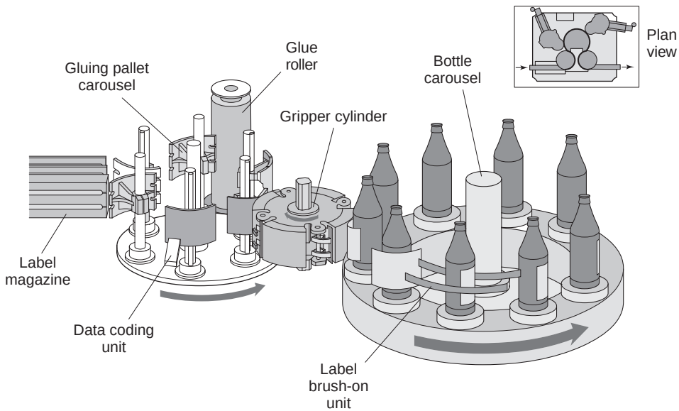
Fig. 21.3 Bottle-labelling station (by courtesy of Krones).
