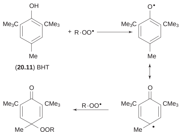
Fig. 20.11 Antioxidant activity of Butylatedhydroxytoluene (BHT).
