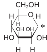
Mannose; \alpha -D-mannopyranose
