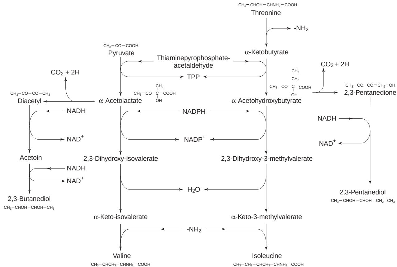
Fig. 12.21 Pathways for the formation and dissipation of the vicinal diketones, diacetyl and 2,3-pentanedione.
