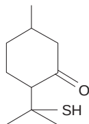
8-Mercapto- p -menthan-3-one (20.12)
