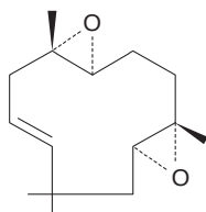
(8.143) humulene diepoxide B
