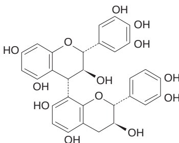
Fig. 4.34 Flavanols, including some that occur in sweet worts.
