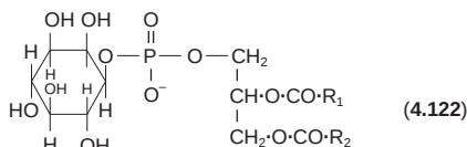
Phosphatidyl inositol
