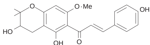
(8.64) dehydrocycloxanthohumol hydrate
