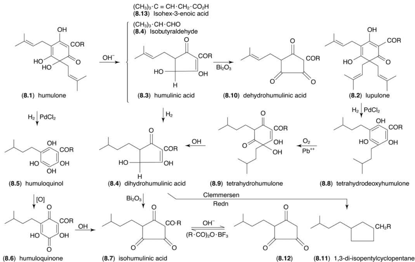
Fig. 8.1 Reactions of \alpha - and \beta -acids.
