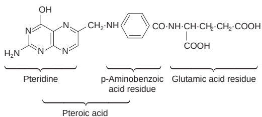
Folic acid
