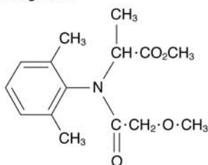
(7.8) Metalaxyl (Ridomil)
