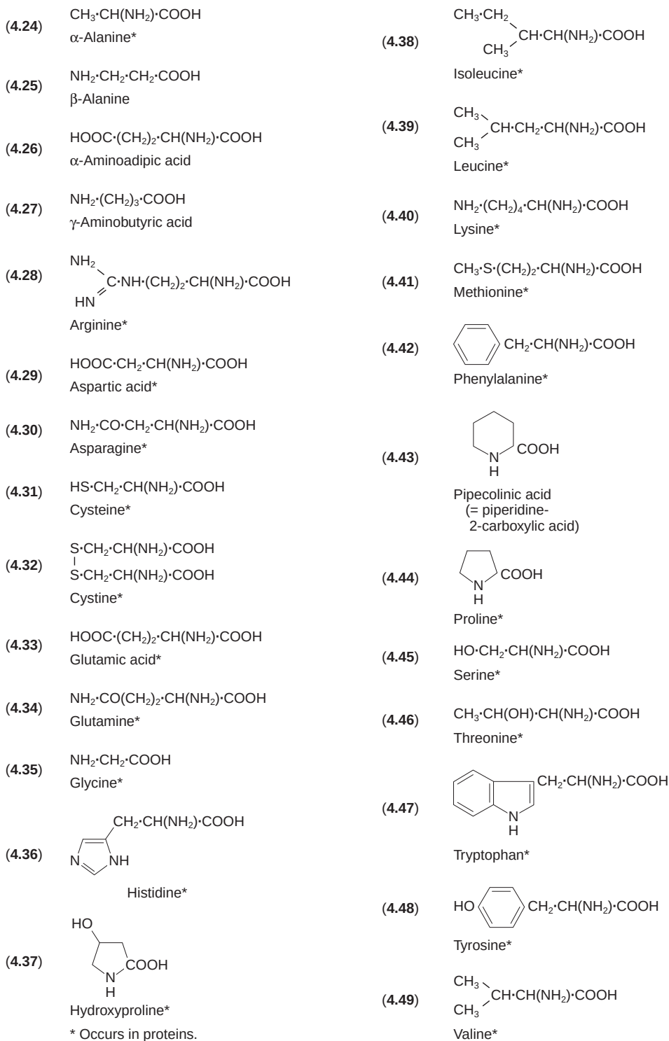
Fig. 4.26 The formulae of most common amino acids and the imino acids pipercolinic acid, proline and hydroxyproline.
