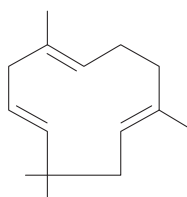
(8.111) humulene
