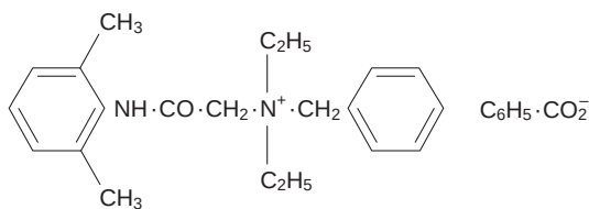
(20.5) Denatonium benzoate
