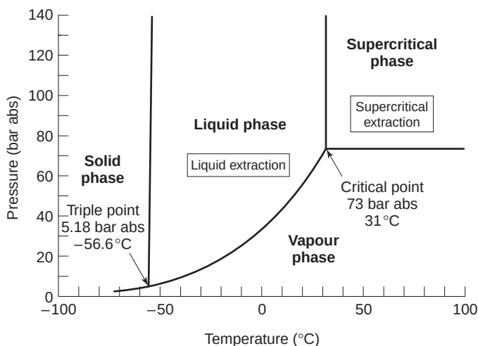
Fig. 7.4 Pressure temperature equilibria for carbon dioxide (Benitez et al. , 1997).
