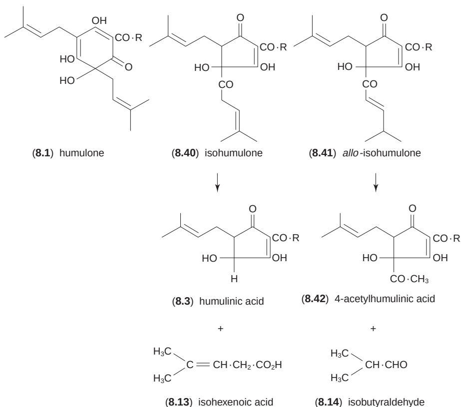
Fig. 8.7 Isomerization and hydrolysis of humulone ( R = \text{Bu}^i without stereochemistry).
