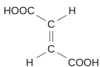
Fumaric acid
