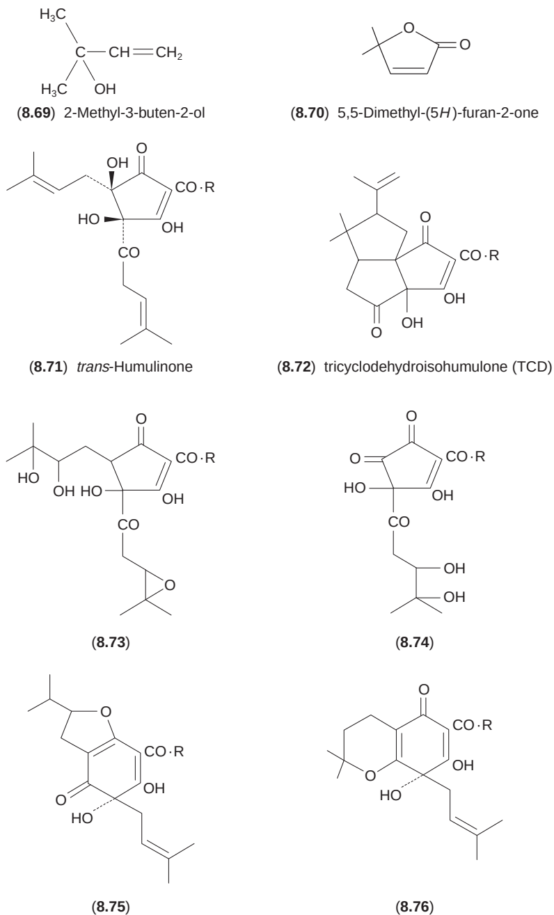
Fig. 8.14 Oxidation products of the \alpha -acids.
