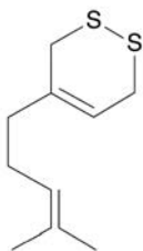
(8.167) 4-(4-methylpent-3-enyl)- -3,6-dihydro-1,2-dithiane
