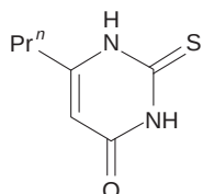
(20.4) Propylthiouracil
