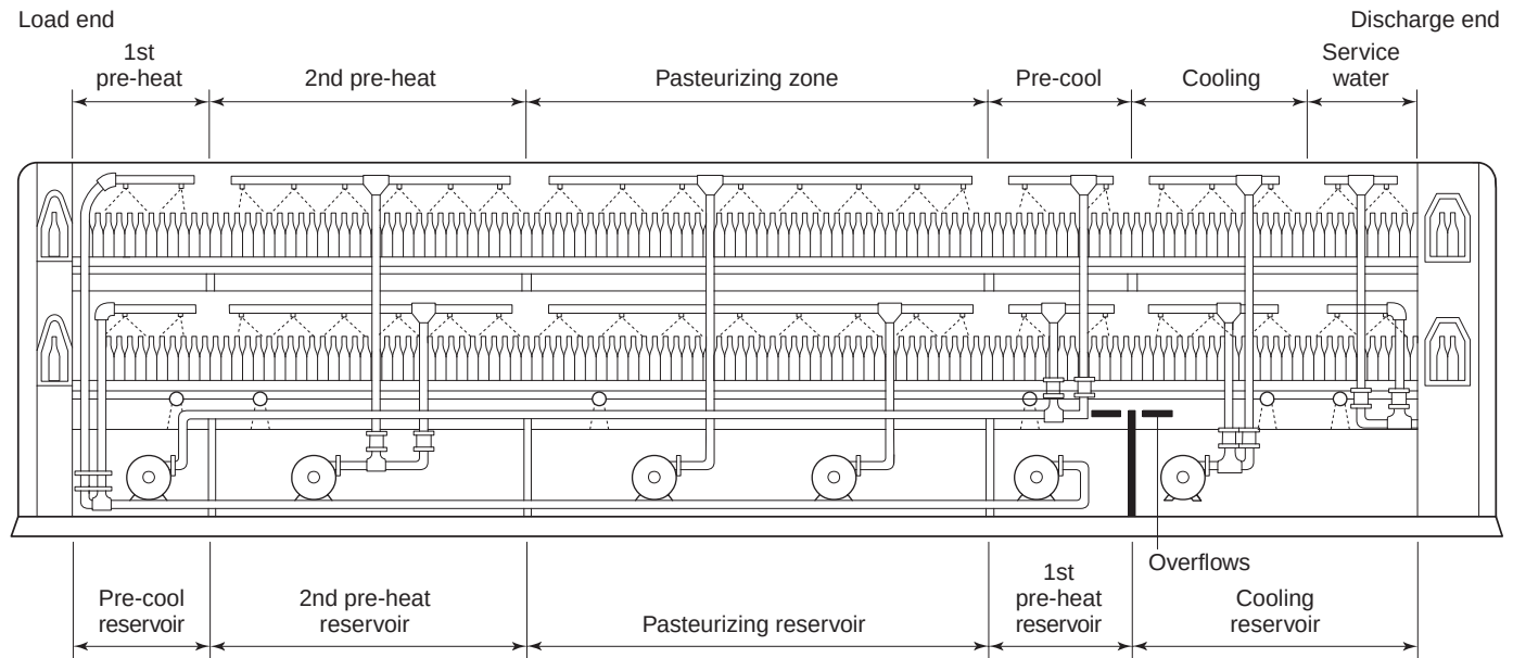
Fig. 21.9 General arrangement of a double-deck tunnel pasteurizer. Times and temperatures for the various zones: 1st pre-heat, 5 min. at 35–50°C; 2nd pre-heat, 13 min. at 50–62°C; Pasteurization, 20 min. at 60°C; Pre-cool, 5 min. at 60–49°C; Cool, at 49–30°C; Discharge, 2 min. at 30–20°C. For can pasteurization the pre-heat and cooling zones may be shortened in length and therefore the beer spends less time in these zones, because of the lower structural strength of the can (Hough et al. , 1982).
