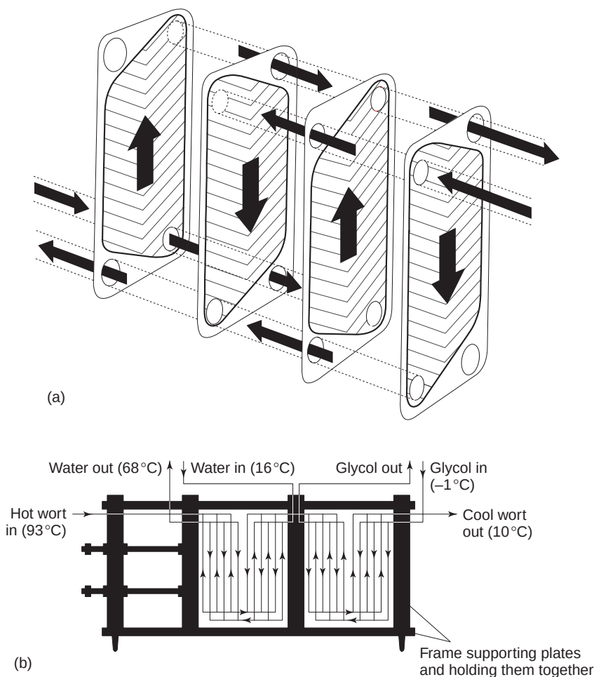
Fig. 10.24 (a) The principles of a plate and frame heat exchanger, indicating the movement of the liquid to be cooled and the counterflow of the cooling refrigerant (Hough et al. , 1982). (b) The flows in a two-stage cooling system (after Hough, 1985). In the first stage wort is cooled by a counterflow of water, which is heated in the process. In the second stage the wort is cooled further by a chilled glycol refrigerant.
