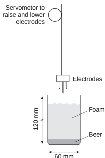
Fig. 19.7 NIBEM foam stability apparatus (after Kloppe, 1973).
