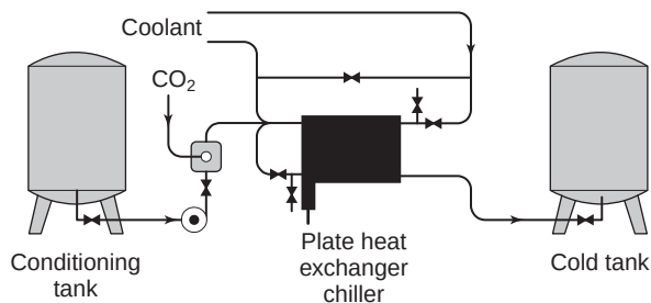
Fig. 15.6 Carbonation and chilling of beer 'on the run', from conditioning tank to cold tank (Hough et al. , 1982).
