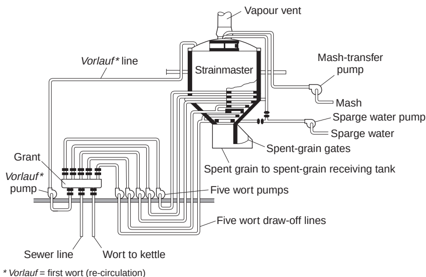
Fig. 6.18 A Strainmaster lauter tun. The patent is owned by Anheuser-Busch (after Briggs et al. , 1981).
