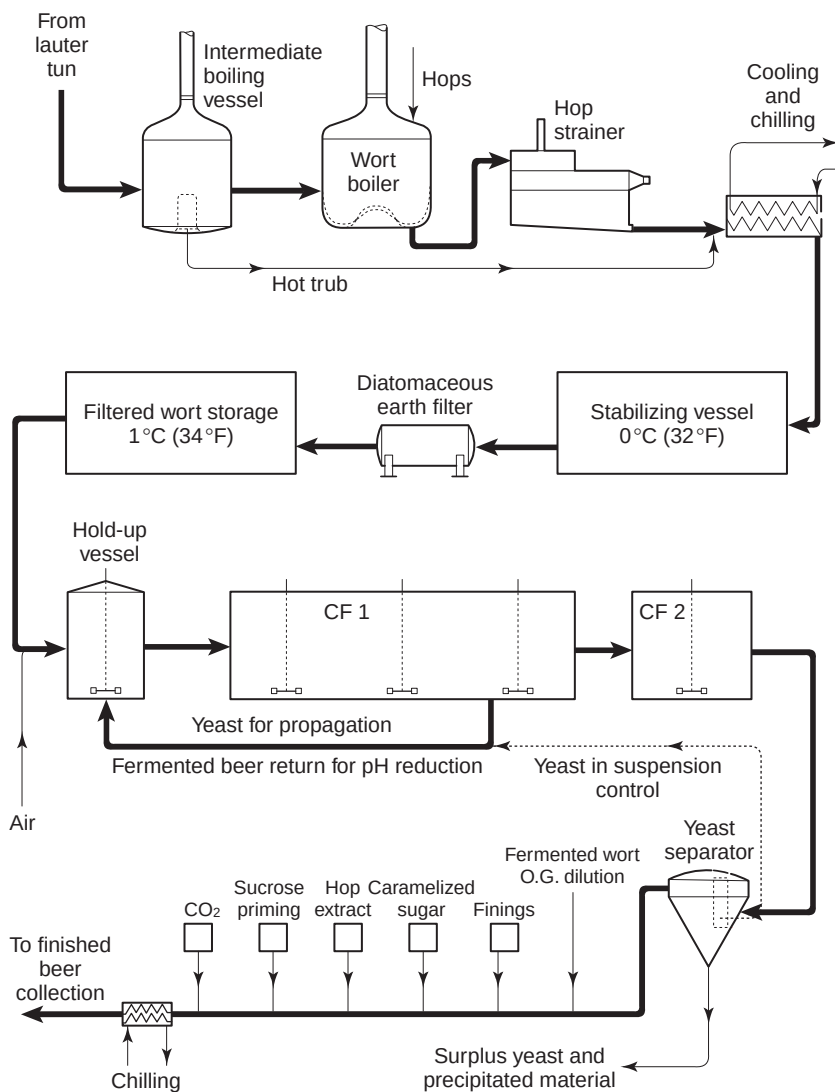
Fig. 14.12 New Zealand system of continuous fermentation, (CF1) continuous fermenter 1, (CF2) continuous fermenter 2 (Courtts, 1957, 1958).
