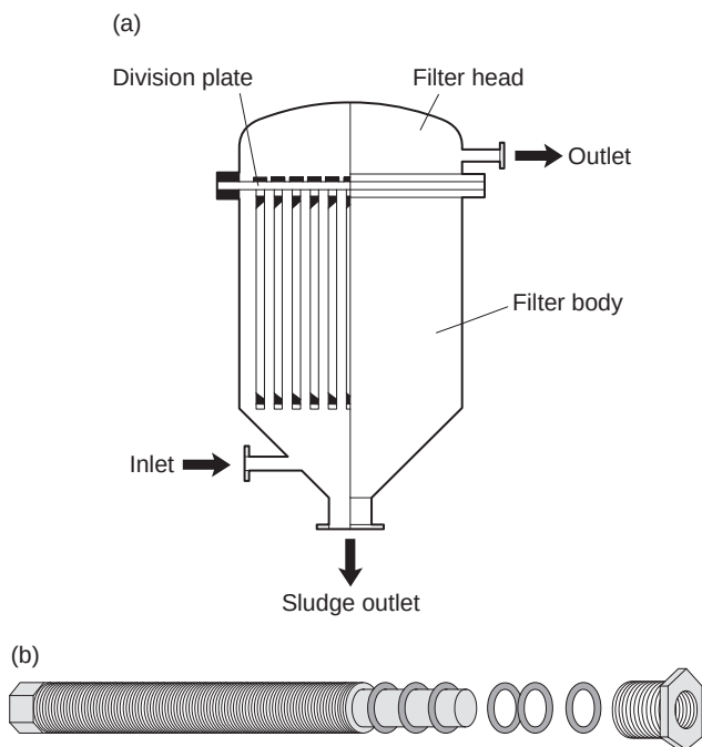
Fig. 15.17 Candle filter or Metafilter; (a) candle filter, (b) detail of single candle (Hough et al. , 1982).
