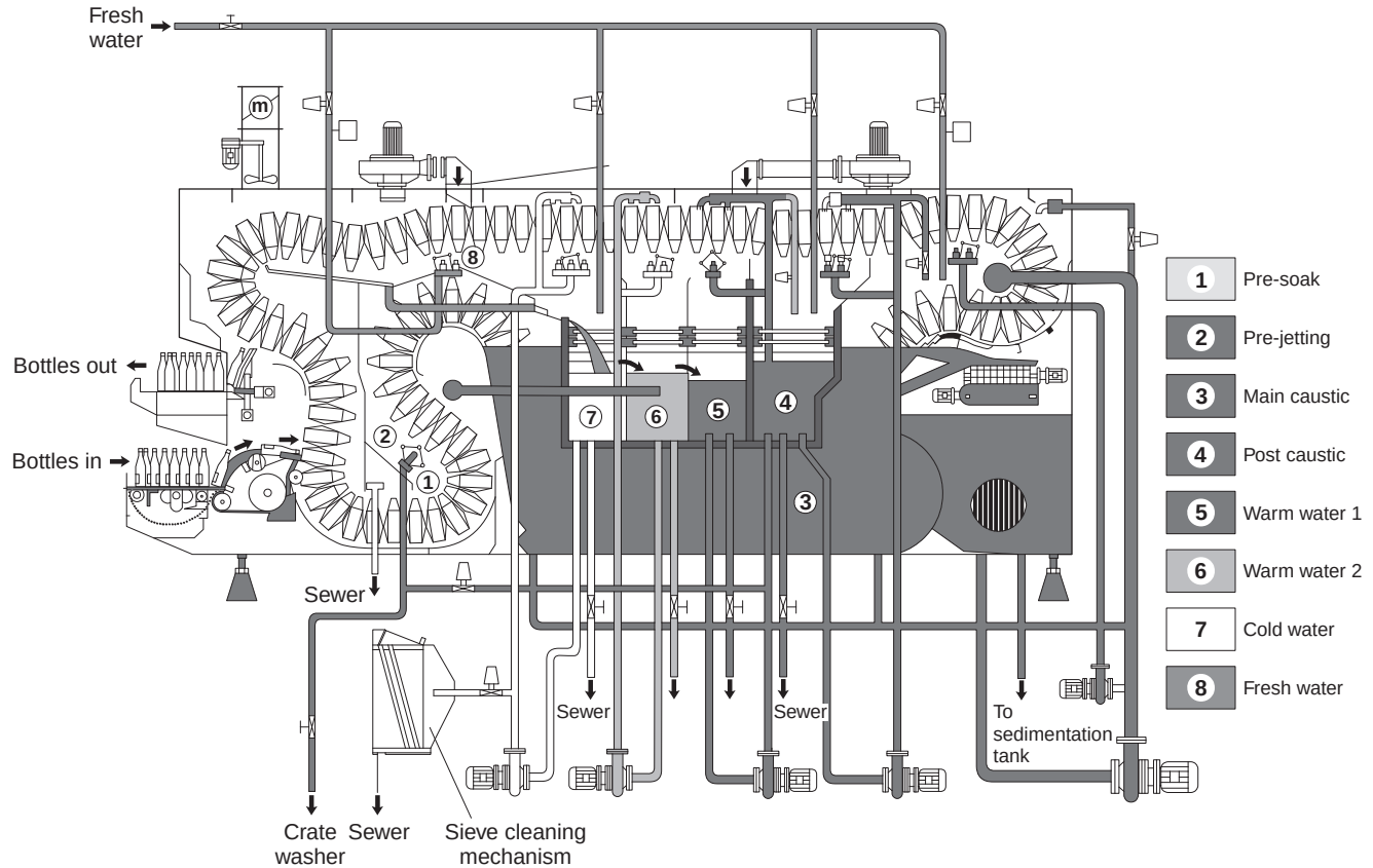
Fig. 21.2 Bottle-washing machine (by courtesy of Krones).
