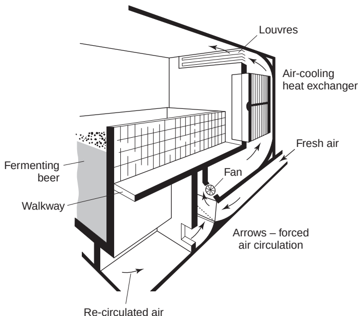
Fig. 14.7 An open square fermenting vessel (after Hough et al. , 1982).
