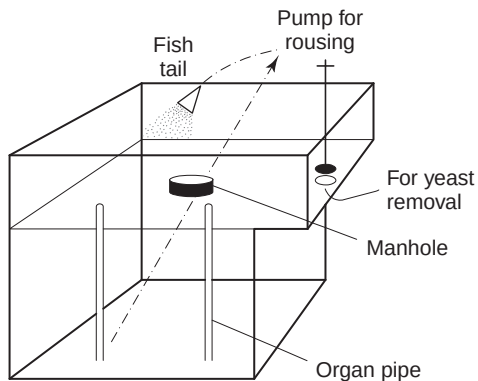
Fig. 14.8 Yorkshire square fermenting vessel (Hough et al. , 1982).
