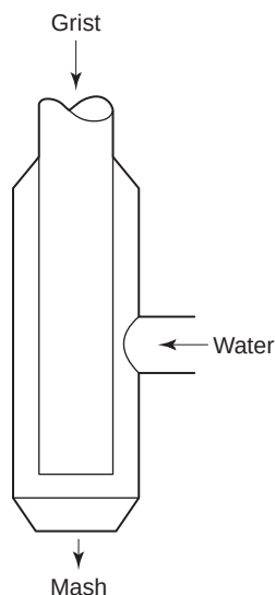
Fig. 6.5 A vortex mash mixer (after Rehberger and Luther, 1994). The grist falls into a swirling tube of liquor from that tangentially injected into the outer chamber. With these, and other pre-hydrators, it is desirable to have a mixing chamber through which the grist must pass before it leaves the unit.
