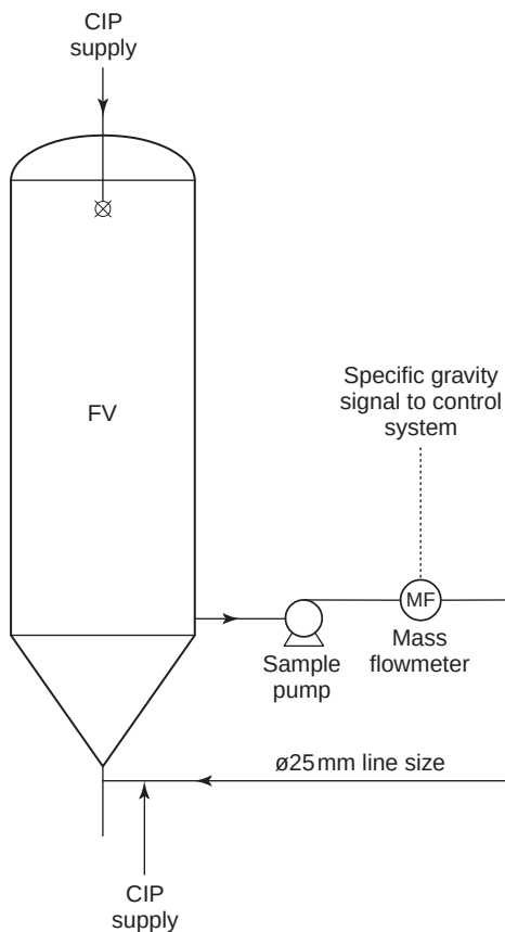
Fig. 14.14 Specific gravity monitoring system using a sample loop; the product sampled is fermenting wort in the specific gravity range 1000–1100 °Sacch, a signal is sent from the mass flowmeter to the control system, sample pump must operate in both directions to allow for CIP; (FV), fermenting vessel (Barnes, 2001).
