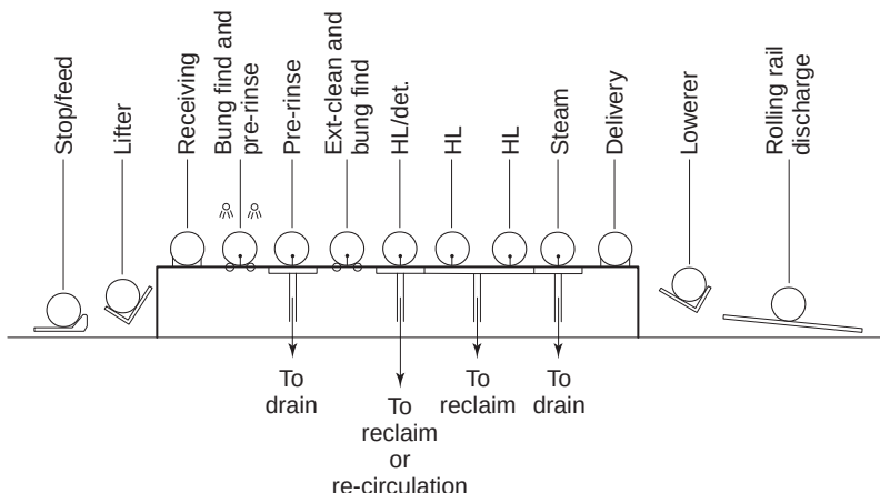
Fig. 21.19 Internal cask washing equipment: nine station chain machine with moving centre beam; HL, hot liquor (water); det, detergent applied to outside of cask (not used in all installations) (by courtesy of Porter Lancastrian Ltd.).
