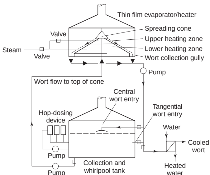
Fig. 10.10 A diagram of a ‘Merlin’ wort boiling system in which the wort is collected in a whirlpool vessel and is heated, boiled and volatiles stripped by pumping it in a thin film over a steam-heated cone in a separate vessel (after various sources, including Anton Steinecker literature).
