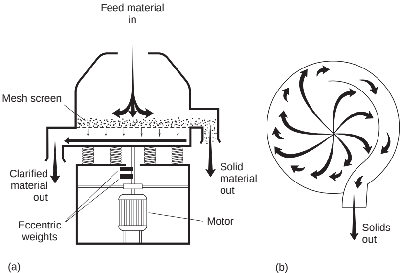
Fig. 10.23 (a) A vertical section of a vibrating screen filter and (b) the distribution and movement of solids on the filter surface as seen from above (Button et al. , 1977).
