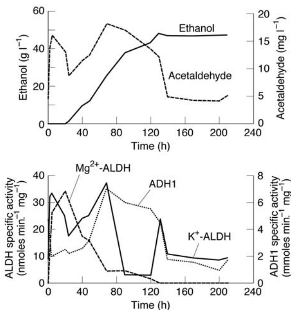
Fig. 12.20 Specific activities of \text{Mg}^{2+} - and \text{K}^{+} aldehyde dehydrogenases (ALDH), alcohol dehydrogenase (ADH1) and changes in the concentrations of acetaldehyde and ethanol during a stirred 2.5 litre laboratory anaerobic fermentation using 12°P lager wort and a lager yeast strain (W. Tessier, unpublished data).
