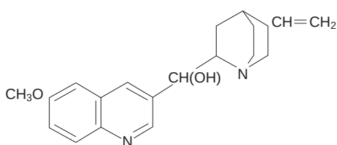
(20.1) Quinine
