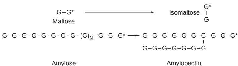
Fig. 4.19 A summary of how the enzymes, that together make up diastase, act on the polysaccharide components of starch or their breakdown products (after Briggs, 1998). G, \alpha -D-glucopyranose residues – , (1,4)-link |; (1,6)-link; *, reducing group.
