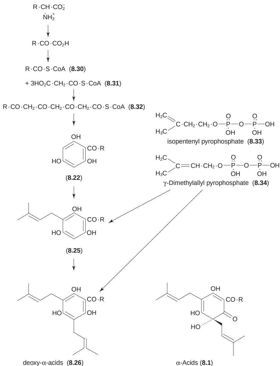
Fig. 8.3 Biosynthesis of the \alpha -acids.
