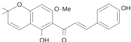
(8.63) dehydrocycloxanthohumol
