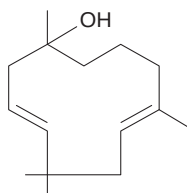
(8.146) humulol
