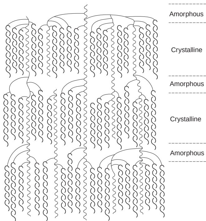
Fig. 4.18 A diagram of the ways in which amylopectin molecules may be packed together in a starch granule to create amorphous and crystalline regions, which differ in their susceptibilities to enzymolysis (after Imberty et al. , 1991). Many of the side chains are wound together in double helices. The single reducing chain end is at the top of the diagram. Linear amylose molecules, some of which are in the form of helices and inclusion compounds with polar lipids are, in some way, interspersed with the amylopectin in the granules, possibly in the amorphous regions.
