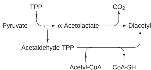
Fig. 17.5 Pathways for the formation of diacetyl by lactic acid bacteria.
