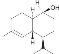
(8.125) T-Cadinol
