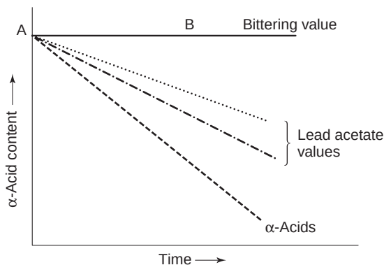
Fig. 8.13 Schematic diagram of the changes in resin content and bittering value of hops during storage (Whietar, 1965, 1966).
