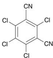
(7.13) Chlorothalonil
