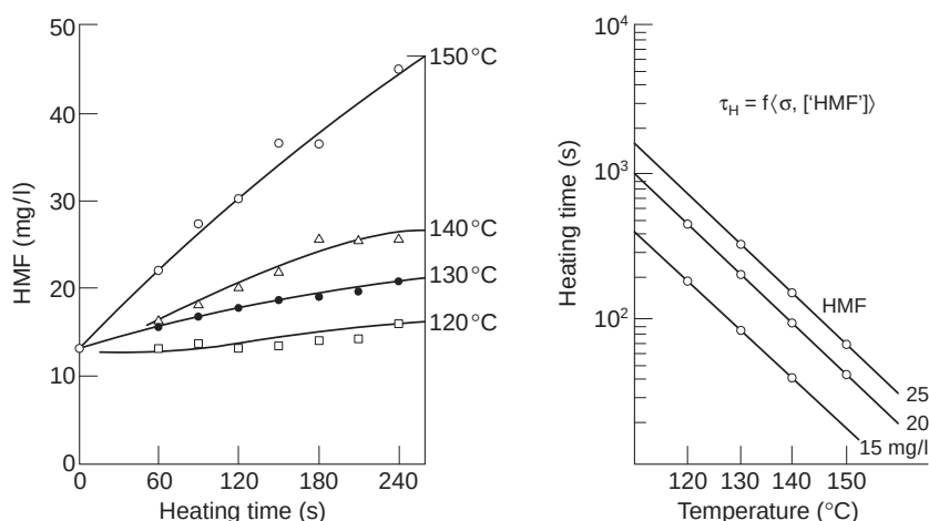
Fig. 9.2 Hydroxymethylfurfural production during high temperature boiling (Miedaner, 1986).
