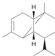
(8.119) copaene
