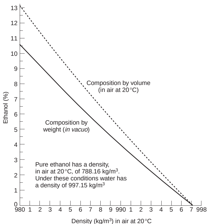
Fig. A1 The relationships between the densities ( \text{kg/m}^3 ) of alcohol (ethanol)/water mixtures, by volume in air at 20°C, or by mass in vacuo . Data from the Brewing Room Book , 1998–2000, p. 281, Pauls Malt, Ipswich and Kentford, Suffolk, UK.
