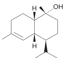
(8.123) δ-Cadinol
