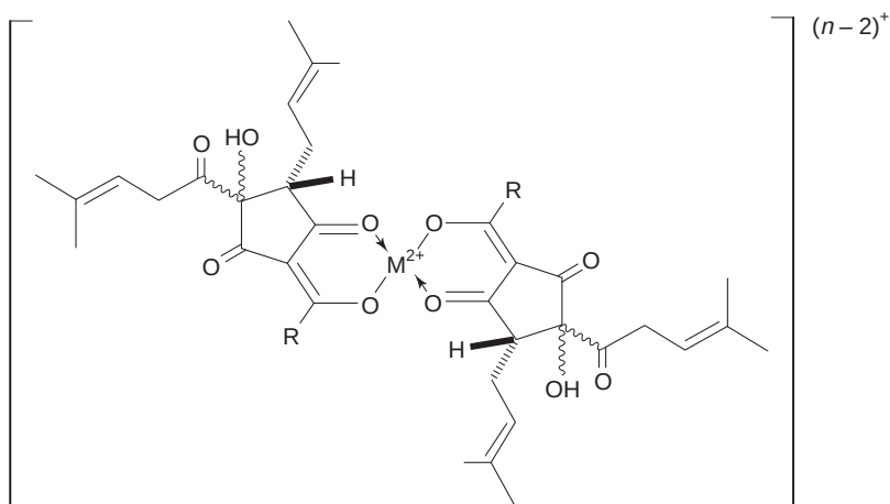
Fig. 19.8 Possible structure of iso- \alpha -acids chelated to a metal cation (Baxter and Hughes, 2001, Fig. 2.2 ). Reproduced by permission of The Royal Society of Chemistry
