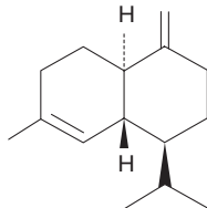
(8.121) γ-Cadinene
