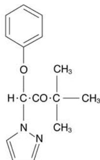
(7.12) Tridimefon (Bayleton)
