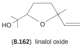
Fig. 8.24 Oxygen heterocyclic compounds in hop oil.
