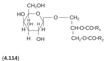
Mono-β-D-galactosyl diglyceride
