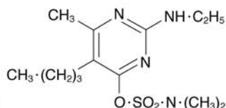
(7.15) Bupirimate (Nimrod)
