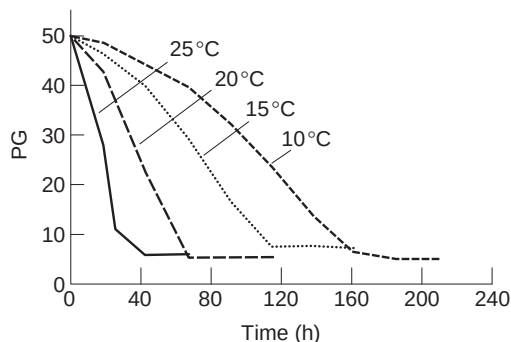
Fig. 13.3 Effect of temperature on fermentation rate. Fermentations were performed at the temperatures indicated using pilot scale 8 hl cylindroconical fermenters, a lager yeast strain, pitched at a rate of 12 \times 10^6 viable cells/ml into an all-malt lager wort with an OG of 1050 (12.5°P) and an initial dissolved oxygen concentration of 25 mg/l (Boulton and Box, unpublished data).
