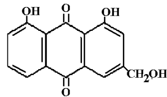
aloe – emodin
