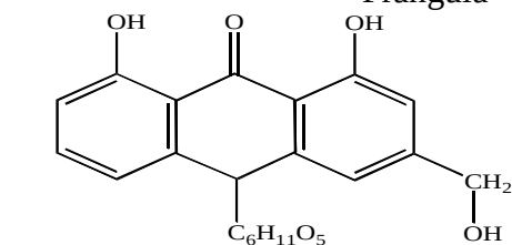
Aloe-emodin-anthrone glycoside
