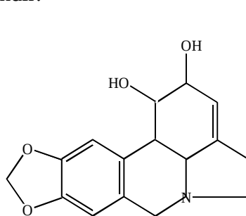
Likorin
