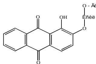
Ruberitric acid
