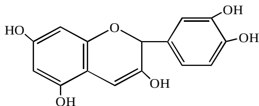
Tsianidin
