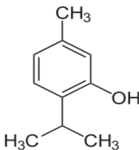
Timol
