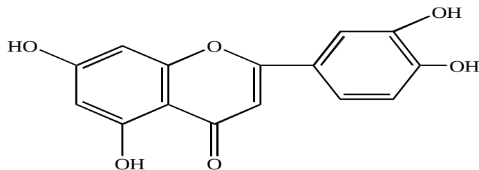
Luteolin
