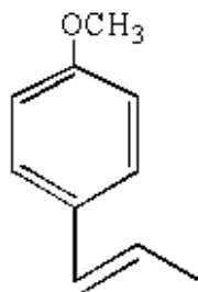
Anetol
