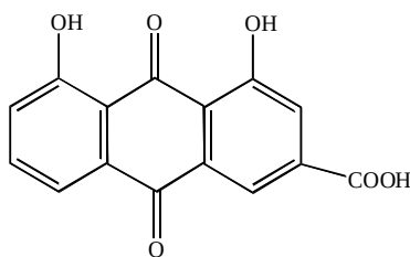
Rein
