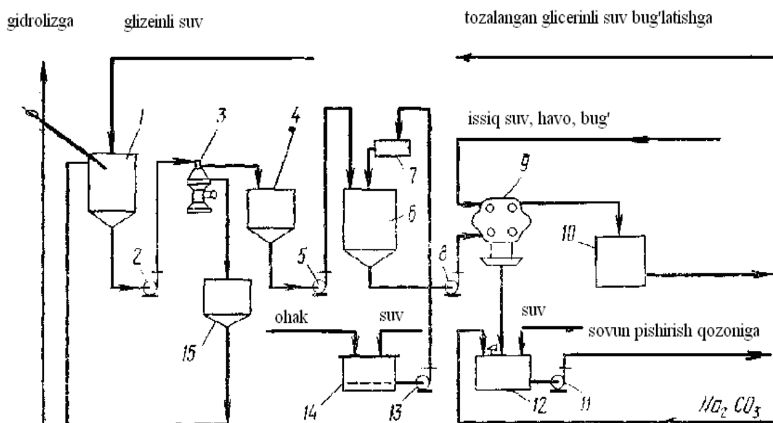
Figure 10.6. Technological scheme of purification of glycerin water
