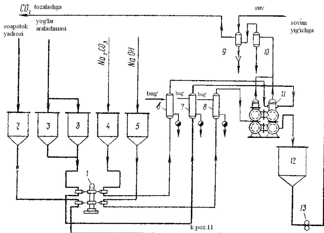
Figure 14.4. Scheme of preparation of household soap base, with continuous method in the TNB-2 device.
