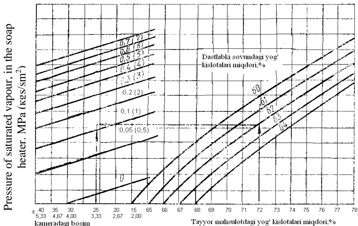
Figure 14.5. The nomogram of determining of soap drying conditions
