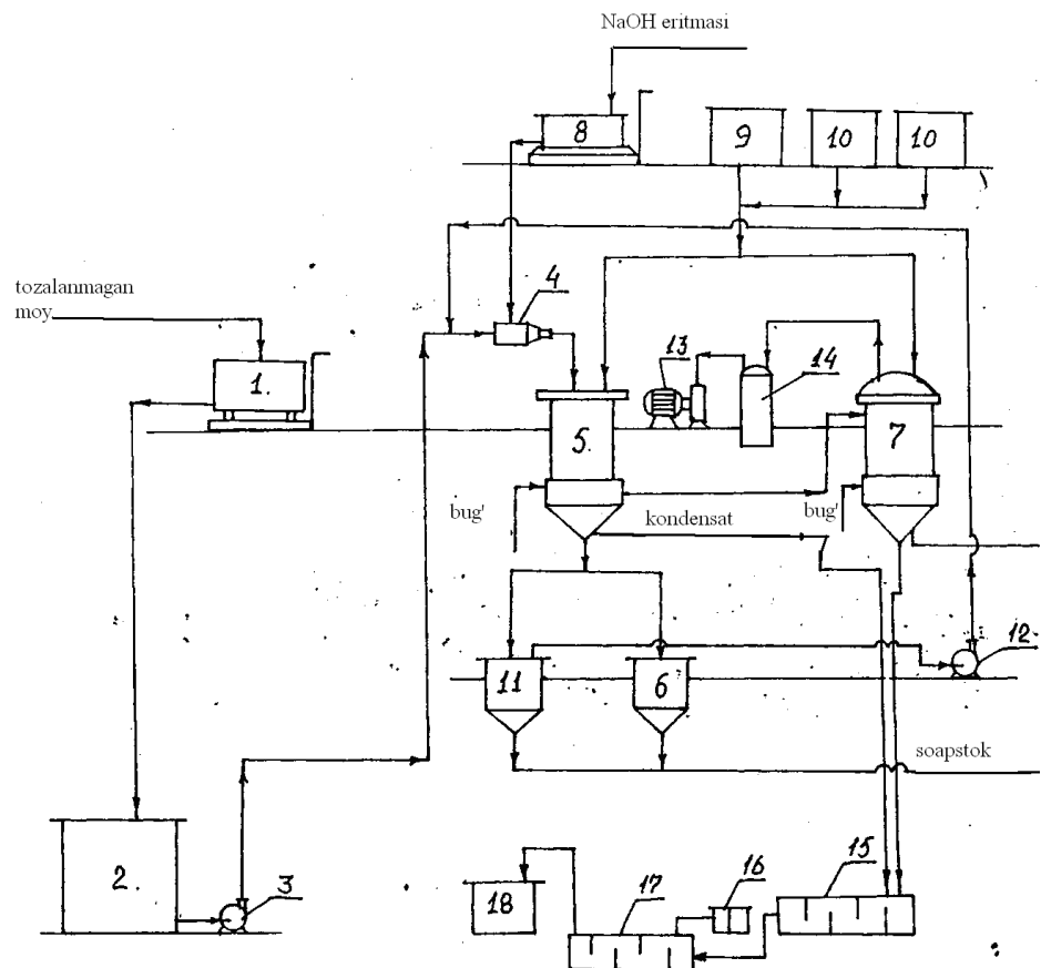
Figure 4.1 Technological scheme of periodic refining processes
