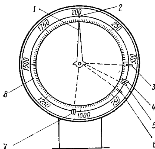
Figure 8.2. The diagram of the head part of the weighted dial scales
