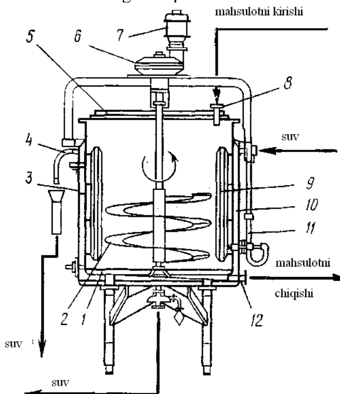
Figure 8.3. Diagram of vertical cylindric mixer.
