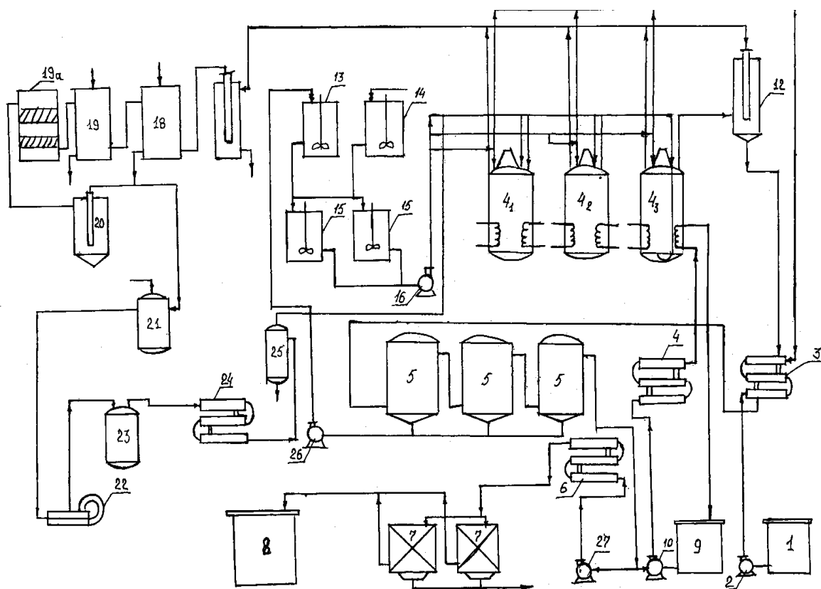
Picture 7.2. Technological scheme of continuous hydrogenation
