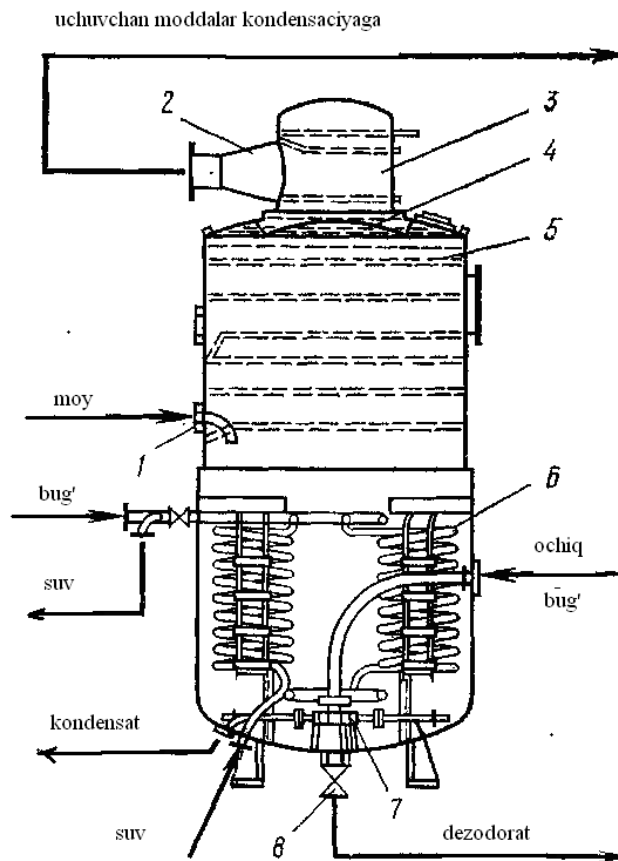
Figure 5.3. Periodic deodorizer
