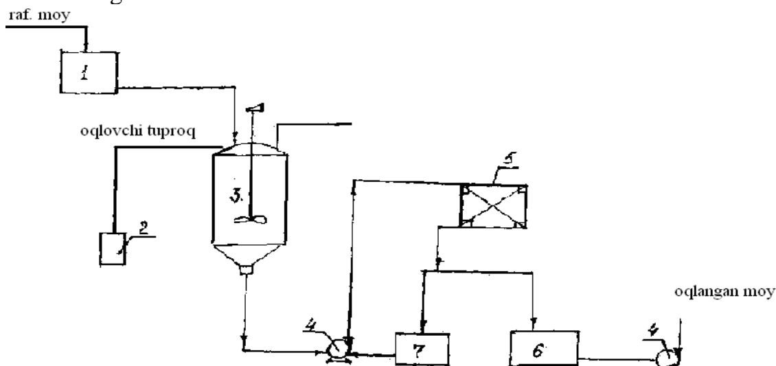
Figure 4.5 Technological scheme of periodic correction of oils.
