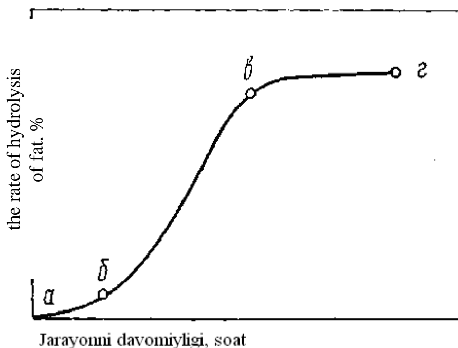
Figure 10.2. Hydrolysis reaction of the fat
