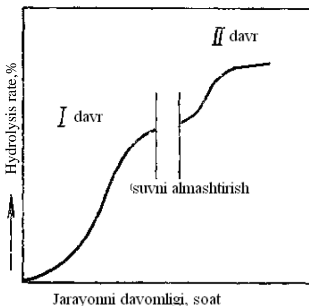
10.3. - picture. Hydrolysis reaction of fat, when worked in two stages
