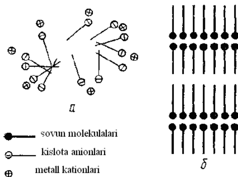
Figure 13.1. Scheme of soap micelle structure
