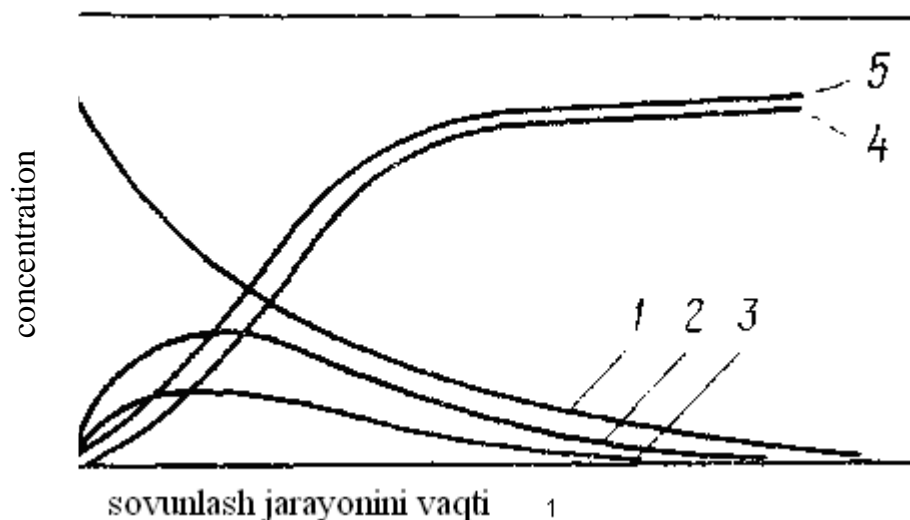
Figure 10.1. Change of glyceride, glycerin and fatty acids in the hydrolysis process:
