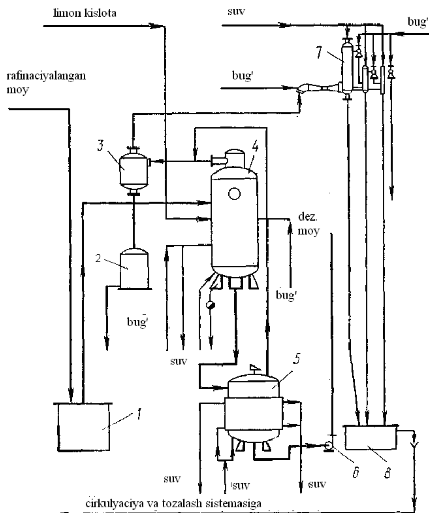
Figure 5.2. Technological scheme of periodic deodorization.
