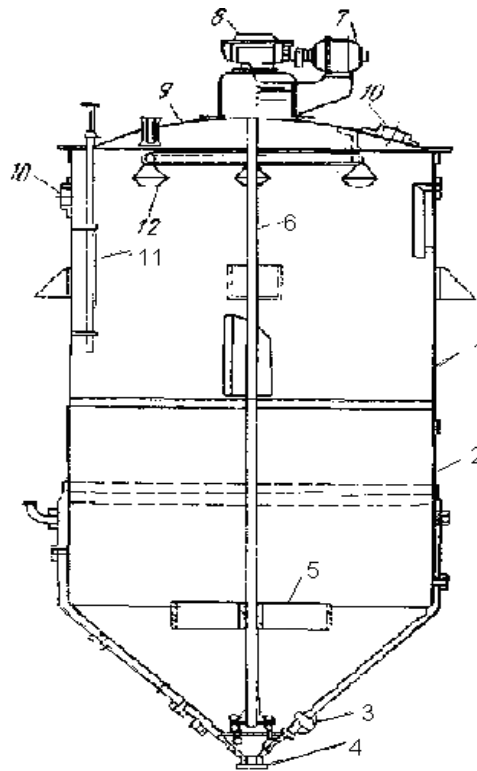
Figure 4.3 Periodic wash and vacuum drying apparatus
