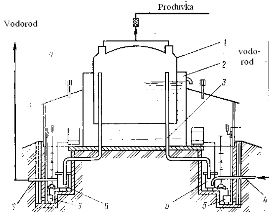
Figure 7.4. Gazholder
