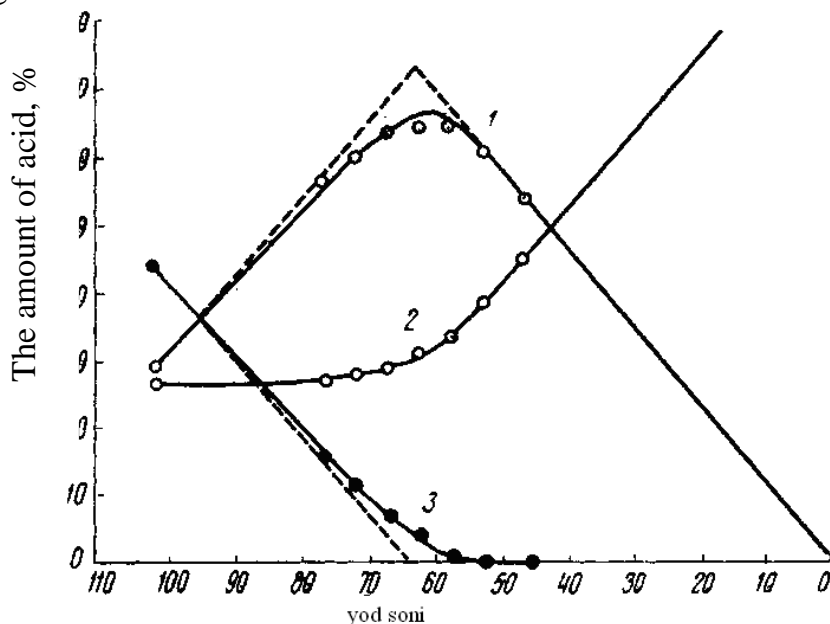
Figure 6.1 Change of fatty acids content in cotton oil hydrogenation: 1-olein, 2-saturated acids, 3-linol
