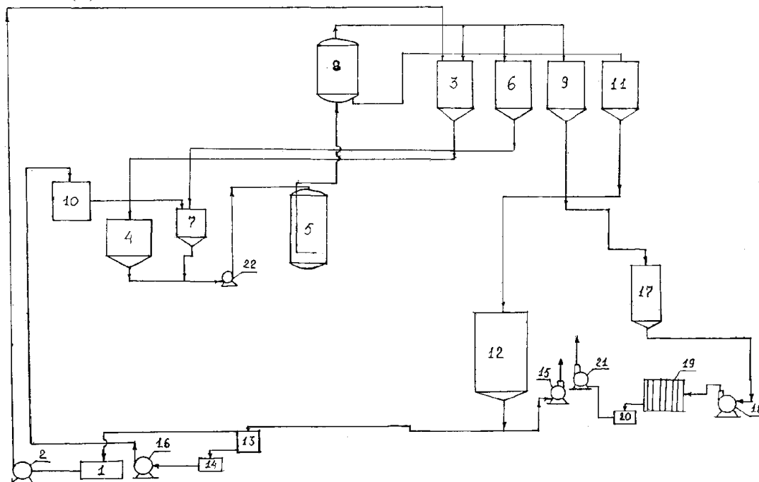
Figure 10.4. Technological scheme of hydrolysis of fat in autoclaves in periodic mode
