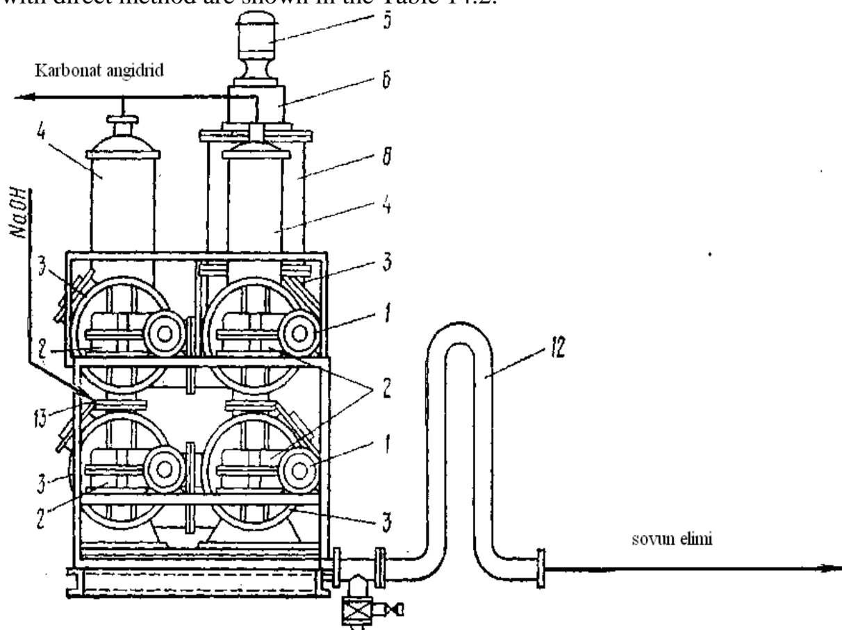
Figure 14.3. Diagram of the TNB-2 apparatus
