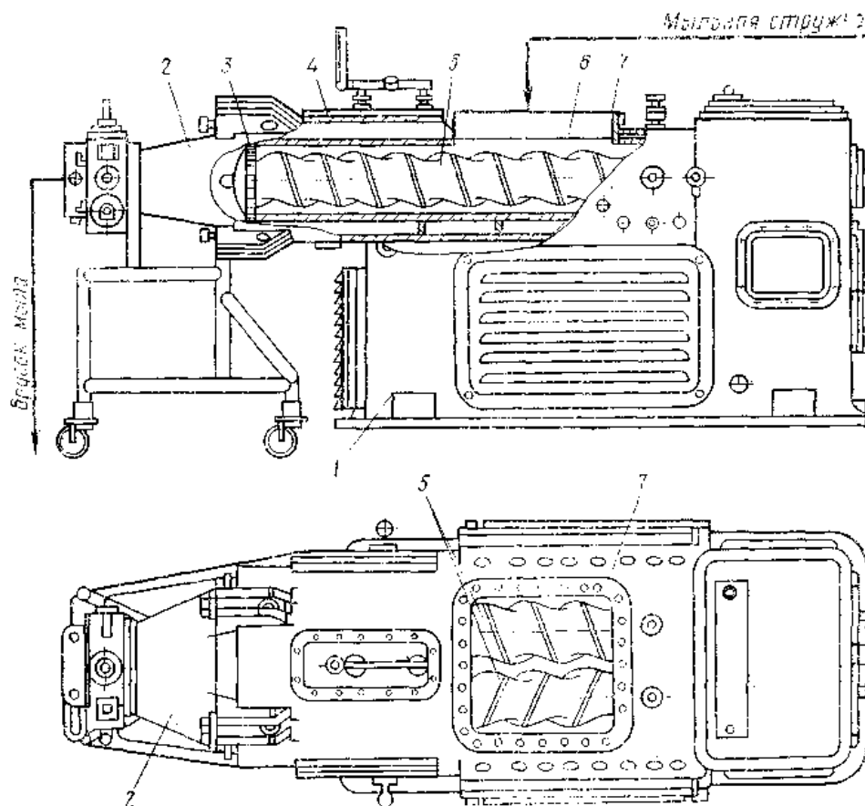
Figure 14.7. Vacuum screw-press
