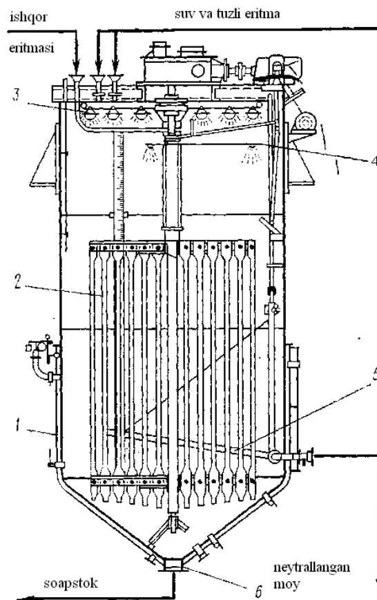
Figure 4.2 Periodic neutralizer
