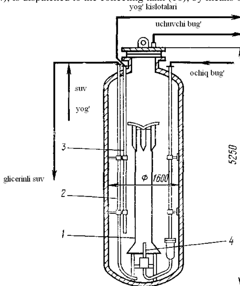
Figure10.5. Hydrolysis autoclave
