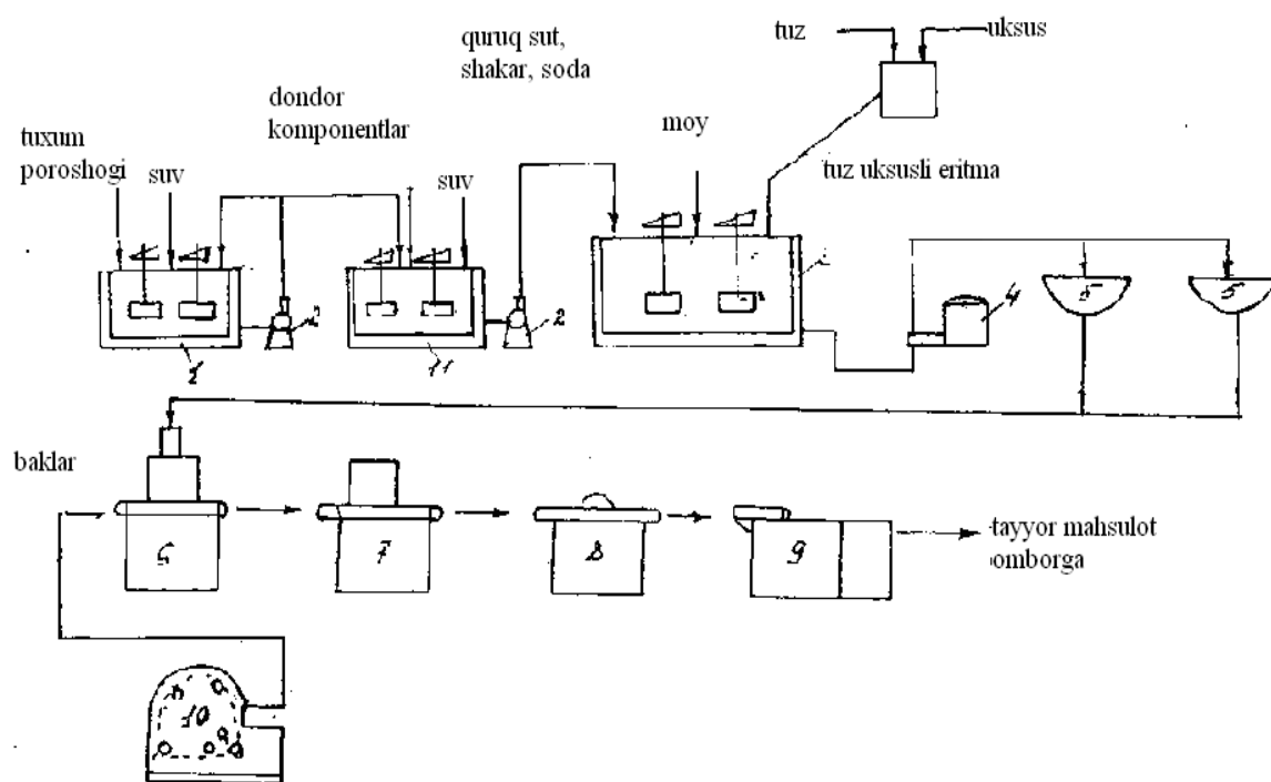
Figure 9.1. Technological scheme of mayonnaise production
