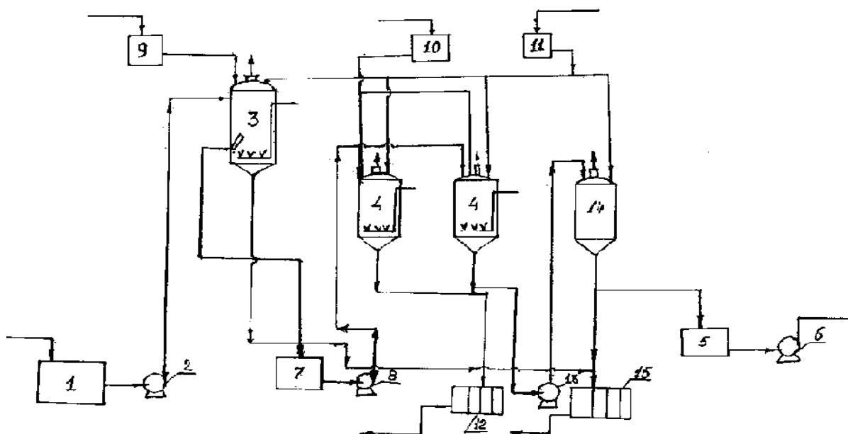
Figure 12.1. Technological scheme for the production of crude fatty acids from soapstock of cotton oil
