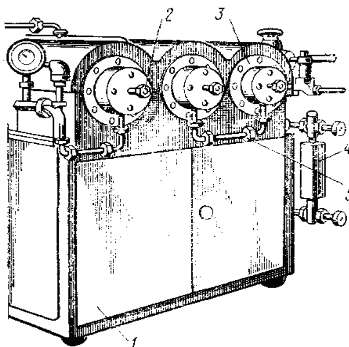
Figure 8.4. Diagram of three-cylindrical extreme-cooler
