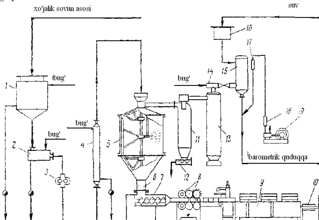
Figure 14.8. Technological scheme of treatment of household soap bases
