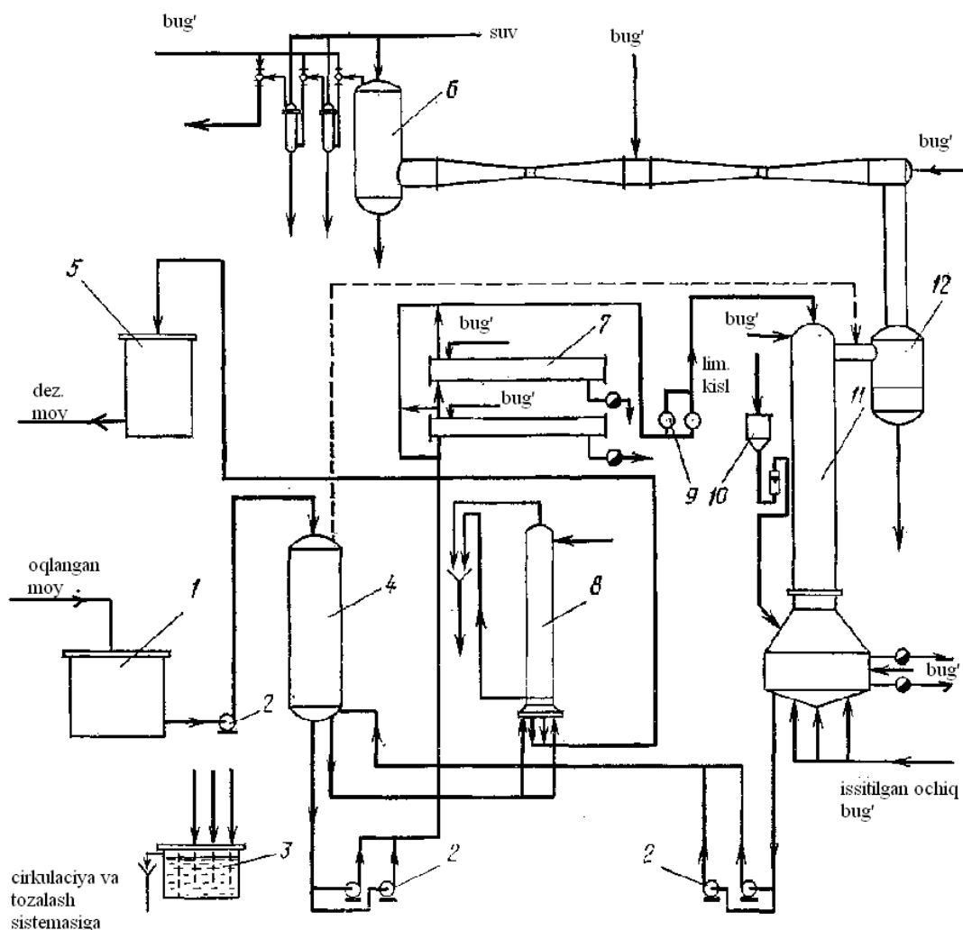
Figure 5.4. Technological scheme of the continuous deodorization on the line A1-MND
