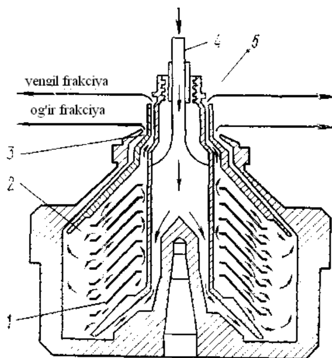
Figure 2.3 Working principle scheme of the separator's separating drum.
