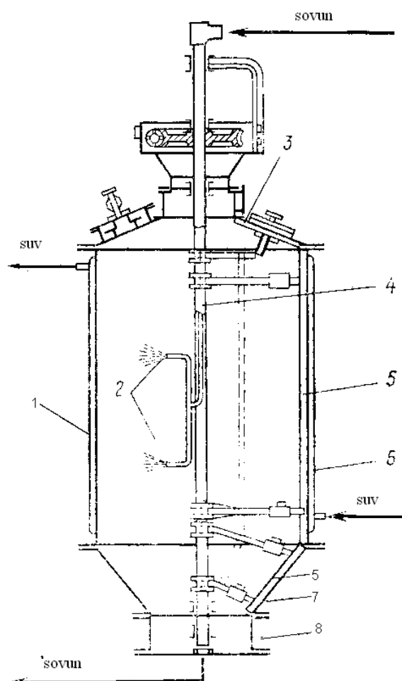
Figure 14.6. Vacuum drying chamber
