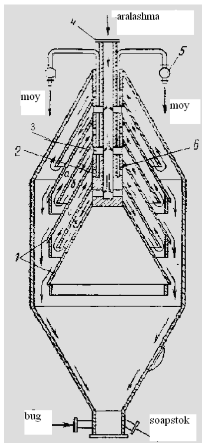
Figure 2.1 Continuous working cutlery - separation circuit diagram
