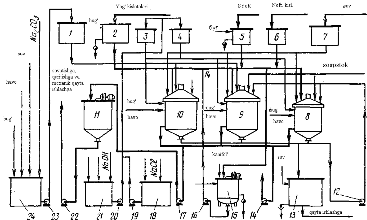
Figure 14.2. Technological scheme of preparation of household soap base on a periodic method
