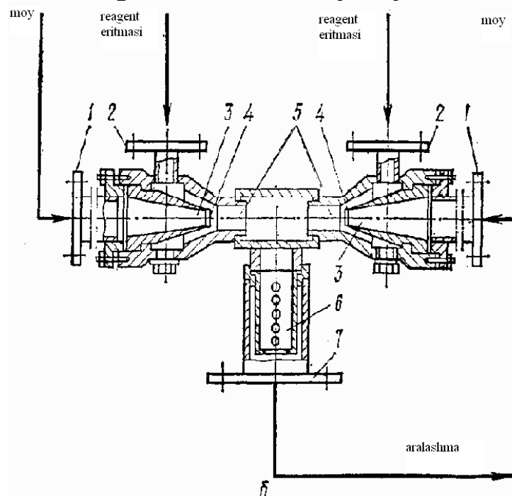
Figure 3.1 The figure below shows the structure of the reactor-turbulier
