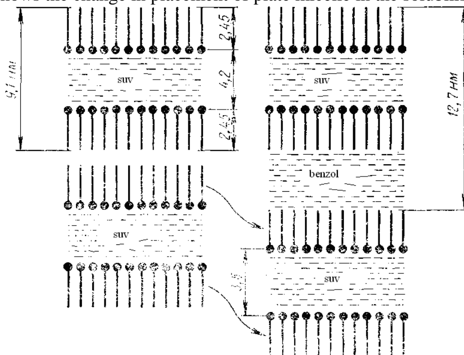
Figure 13.2. The scheme of benzole dissolution in the sodium oleate micelle
