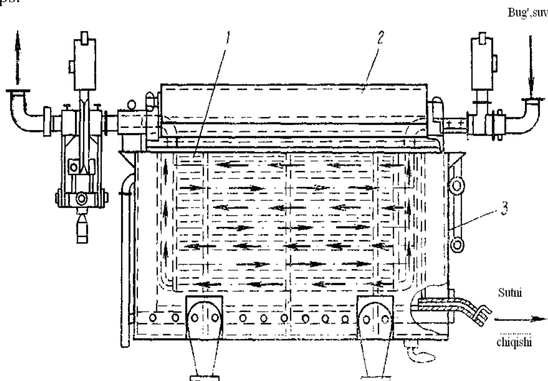
Figure 8.1. The scheme of the fermentation bath
