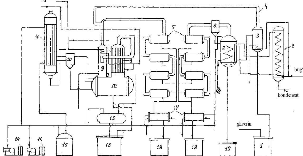
Figure 11.2. Technological scheme of glycerine distillation apparatus
