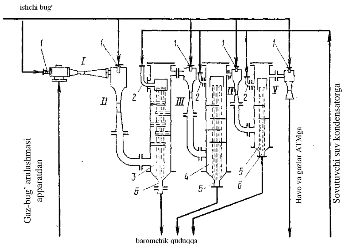
Figure 5.1. A five-stage steam injection vacuum pump scheme
