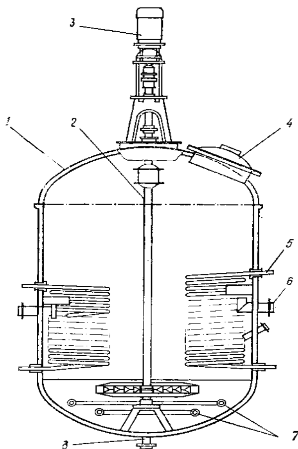
Picture 7.1. Autoclave for hydrogenation of oils
