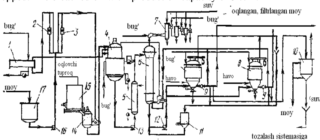
Figure 4.6 Technological scheme of continuous bleaching of oils on DeSmet firmware
