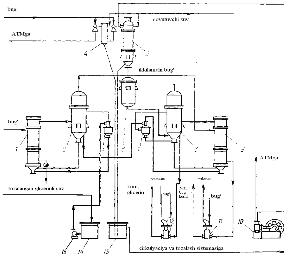
Figure 11.1. Technological scheme of two-body continuous operating device “Podyomnik”
