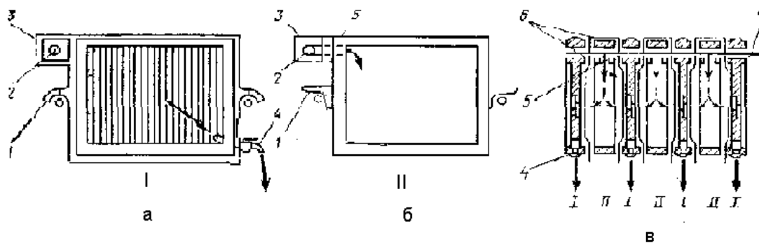
Figure 2.4 Filter-press controls.
