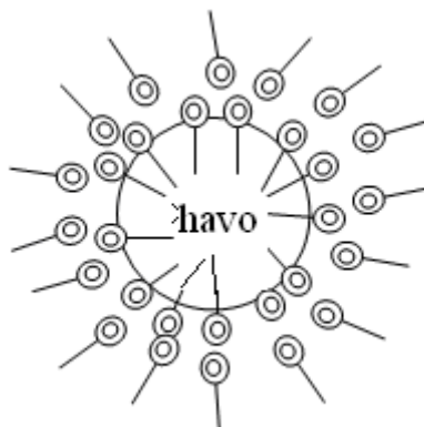
Figure 13.3. The structure of the foam particles
