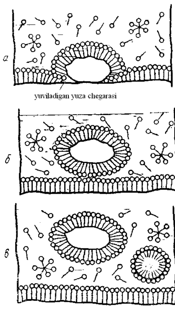
Figure 13.4. Scheme of detergent: a-first stage (wetting of fabric and dirt), b-second stage (disintegration of dirt from fabric), v-third stage (dirt in the stain removal solution)
