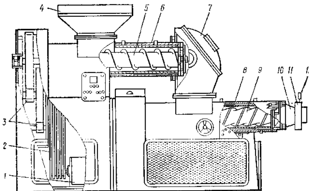
Figure 14.9. Two-stage vacuum screw-press
