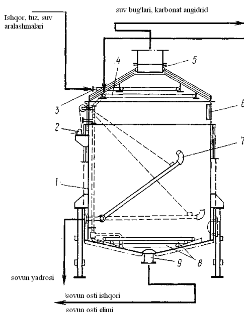
Figure 14.1. Soap cooking pot
