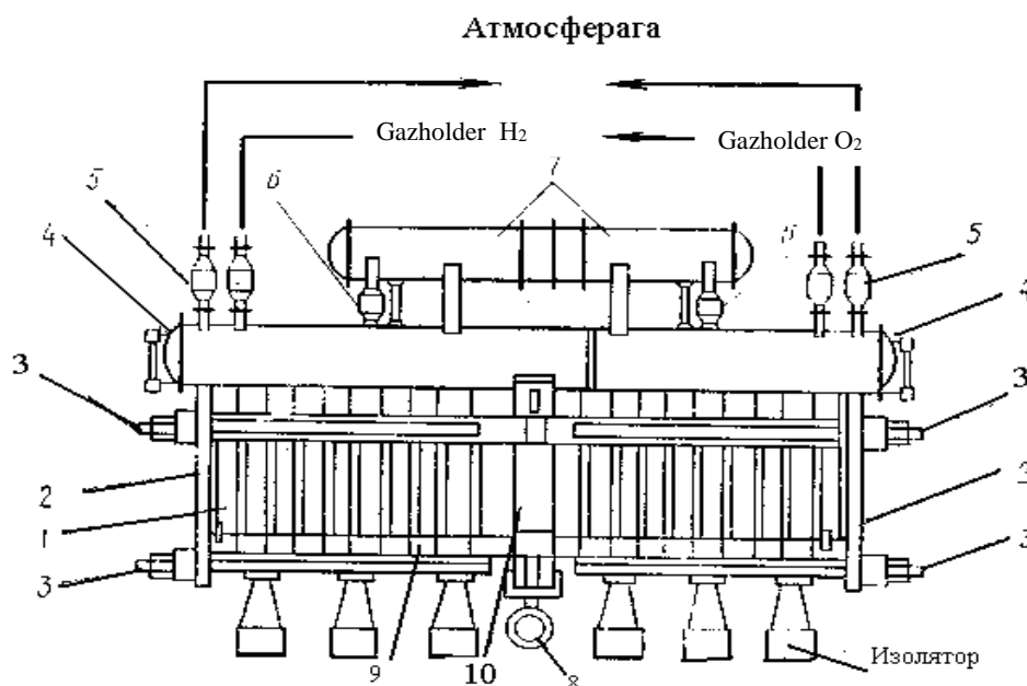
Figure 7.3. Electrolyzer
