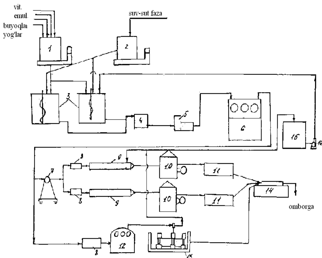
Figure 8.6. Technological scheme of margarine production on line A1-JLU
