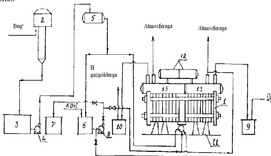
Figure 7.5. Technological scheme of the hydrogen production by electrolytic method
