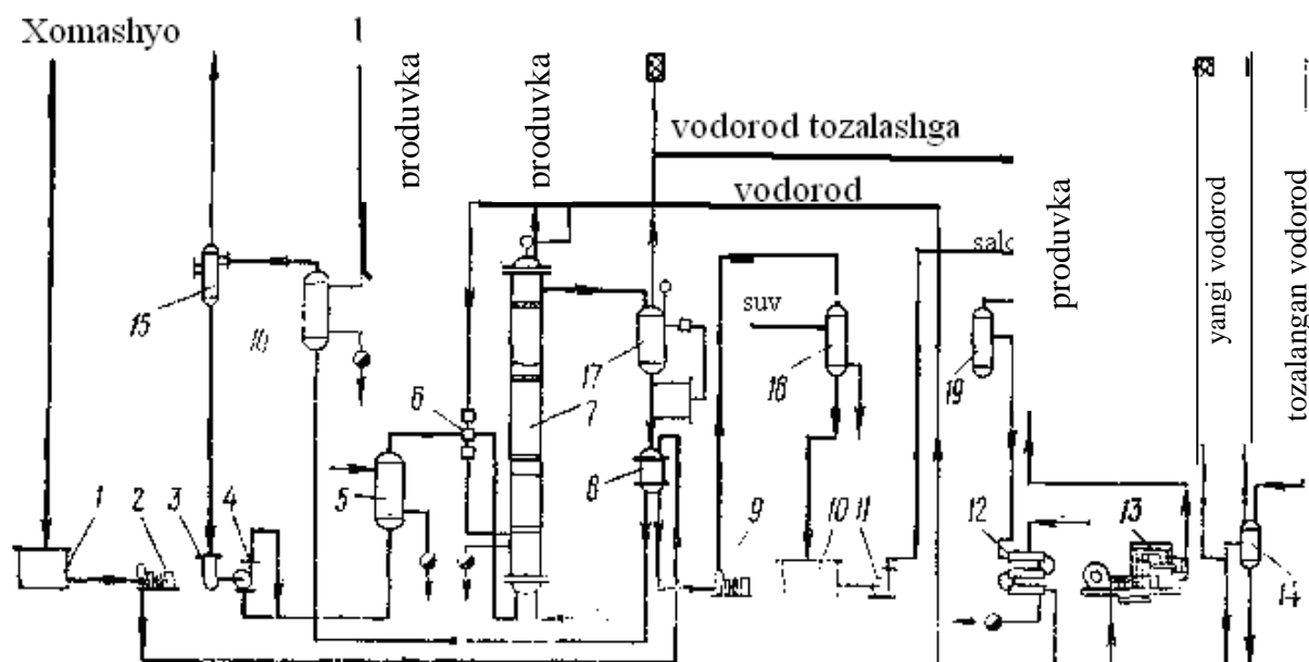
Figure 7.2. Technological scheme of continuous hydrogenation in a stable catalyst pillar reactor.
