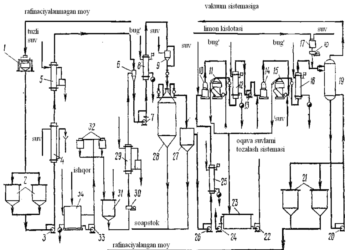
Figure 4.4 Technological scheme of continuous refining of cottonseed oil with emulsive way
