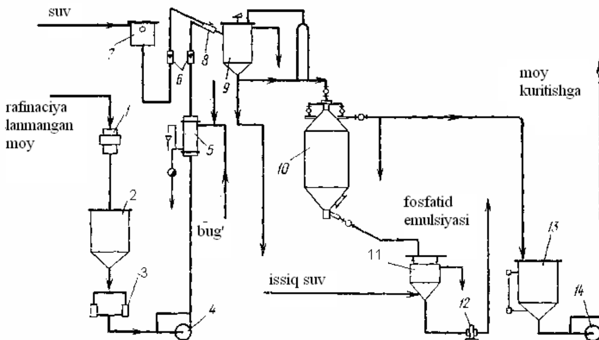
Figure 3.2 Technological scheme of separation of the phases formed during the hydration process in the cutter.
