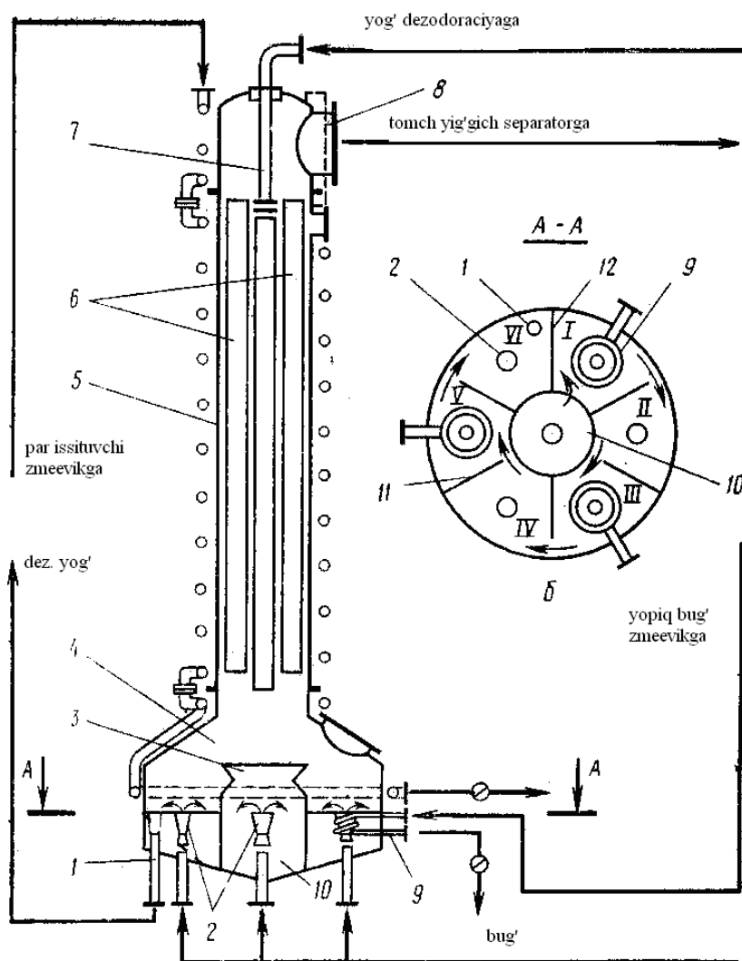
Figure 5.5. Continuous deodorizer
