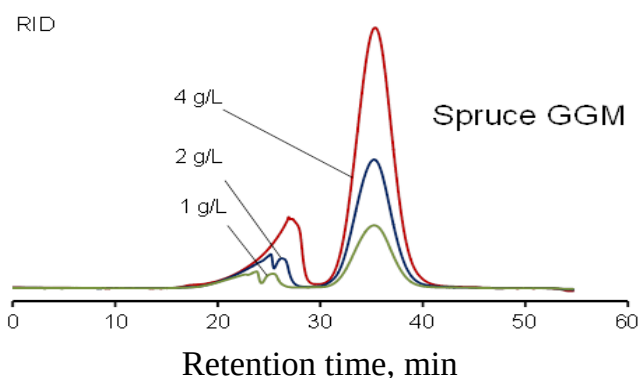
Fig.2 – Elution profiles of galactoglucomannan isolated from spruce wood with hot-water extraction M_w=20 kDa. Eluent: H_2O
