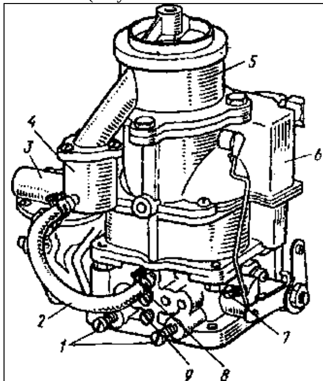
5-rasm. Karbyurator-aralashtirgich K.-91:
