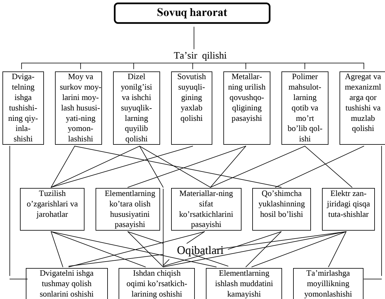
1-rasm. Havoning past haroratini avtomobilga ta'siri
