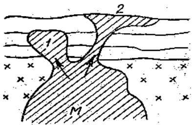
4- rasm. Magmatik jinslarning magmadan hosil bulish sxemasi:
