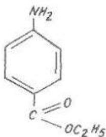
Anestezin – Anaesthesinum
