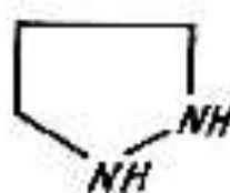
Piraazolidin
