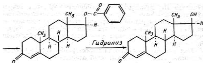
17- benzoattestosteron
