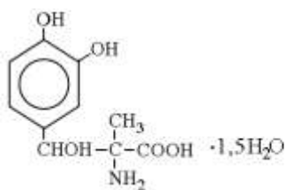
— Methyldopa
