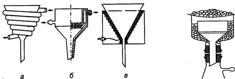
Rasm 6. Voronkalar 1) issiq filtrlash va 2) sovitib filtrlash uchun
