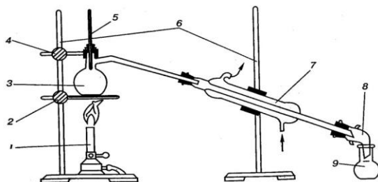
Rasm 1. Suyuqlarni oddiy haydash uchun ishlatiladigan asbob: 1) Bunzen gorelasi, 2) zajim asbest qog'ozi bilan, 3) haydash kolba (Vyurs kolbasi), 4) qisqich, 5) termometr, 6) shtativlar, 7) Libix sovitgichi, 8) allonj, 9) yig'gich kolba
