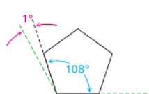
Cyclopentane siklopentan
