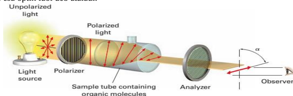
5.3 rasm. Polyarimetrlning shematik ko'rinishi
