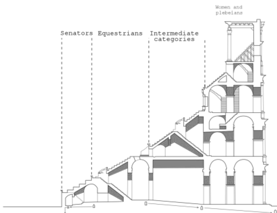
7-rasm Kolizey amfiteatrining qirqimi
