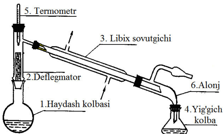
2-rasm. Deflekmtor bilan haydash usuli
