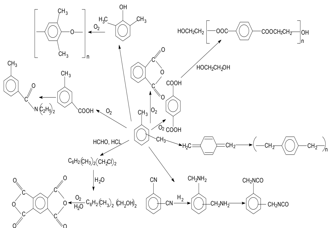
16-rasm. Neftikimyo sanoatida ksilolni ishlatilish sohalari
