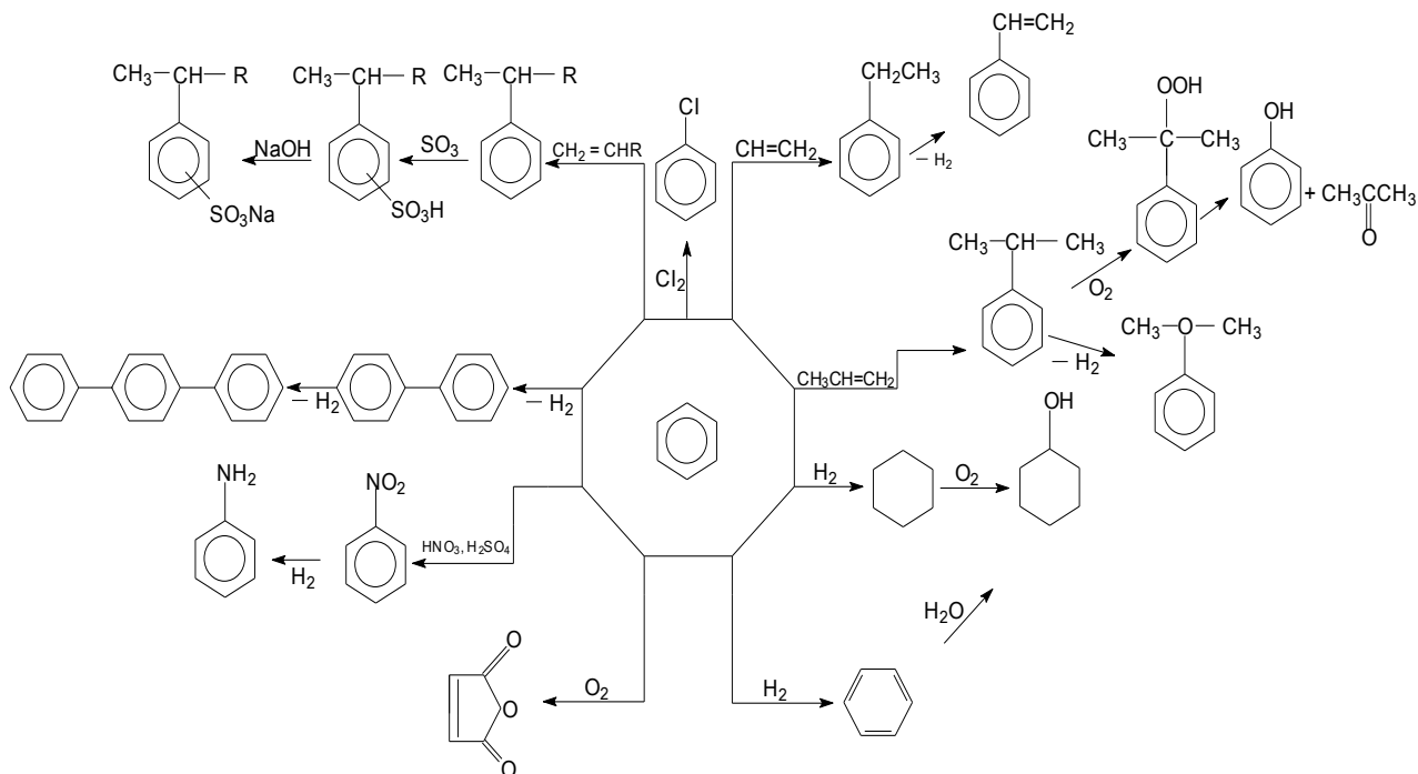
15-rasm. Neftikimyo sanoatida benzolni ishlatilish sohalari
