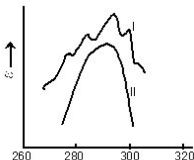
6-rasm. Sirka aldegidining UB spektrlari (I) gaz fazada, (II) spirtda
