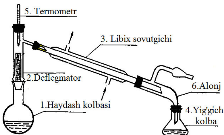
3-rasm. Deflekmator bilan haydash usuli
