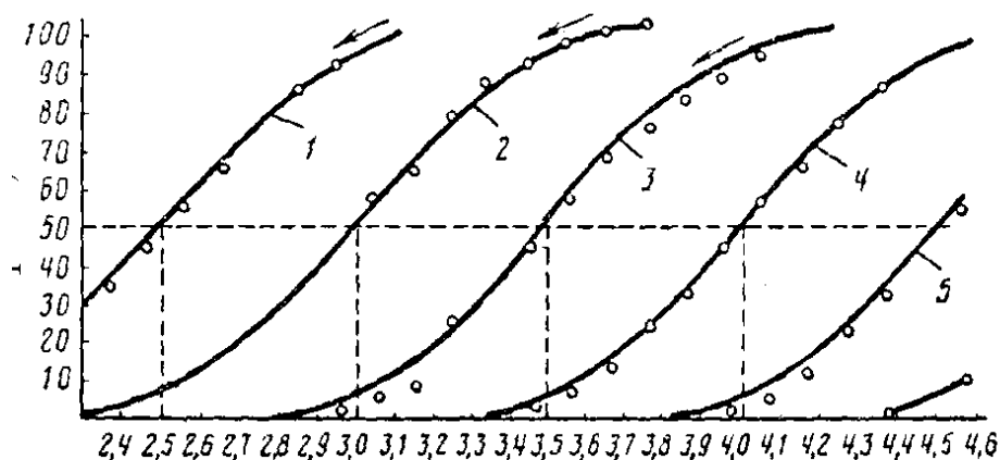
3.20-rasm. Cheprak qalinligini o'rtacha qalinligi 1-2,5; 2-3,1; 3-3,5; 4-4,1; 4-4,6 mm o'zgarganida integral egri chiziqni taqsimlanishi.
