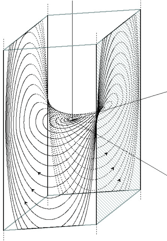
Figure 3. A part of the phase portrait of the system (5)
