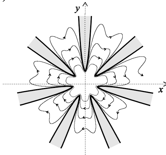
Figure 4. A polynomial system with 7 connectivity components
