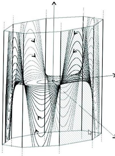
Figure 5. A polynomial three-dimensional with the limit set consisting of eight straight lines
