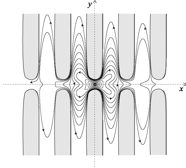
Figure 2. An analytic system with infinite number of connectivity components
