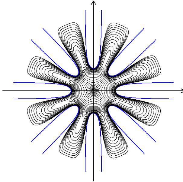
Figure 1. The level line F(x, y) = 0 and one of the trajectories when n = 2 .
