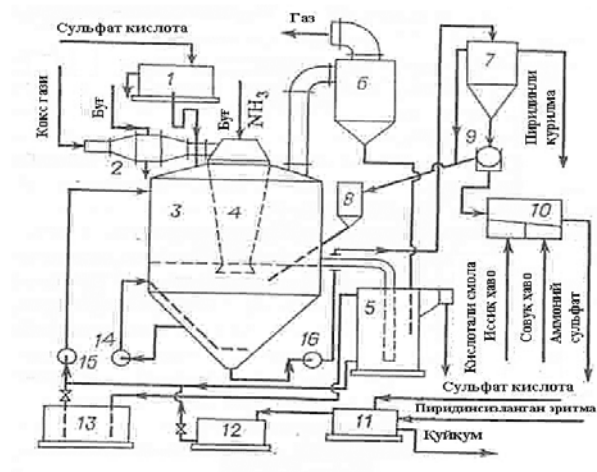
5 – rasm. Ammoniy sulfat ishlab chiqarishning saturatorli usuli tasviri
