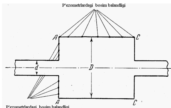
10.1-rasm. Keskin kengayish quvurini tajriba qurilmasi
