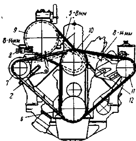
30-rasm. Dvigatellardagi yuritma moslamalarining tarangligini ostlash: a-Isuzu, b-ZMZ-53, v-ZIL-130 1-generator, 2- o'rnatish plankasi, 3-gayka, 4-taranglash roligi, 5-richag, 6-tirsakli val shkivi, 7-generator shkivi, 8- rostlash bolti, 9, 10, 11-kompresor, shamolparrak va suv nasosi, rul boshqarmasidagigidrokuchaytirgich nasosining shkiqlari, 12-taranglash kron-shteyni.
