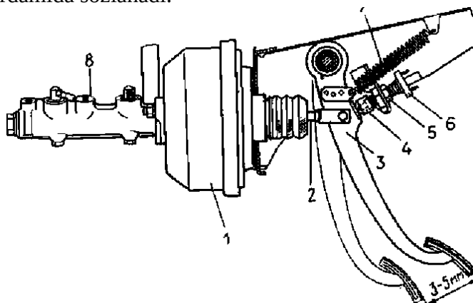
61-rasm. Tormoz tepkisining salt yurish yo'lini sozlash: 1-vakuum kuchaytirgich; 2-itargich; 3-tormoz tepkisi; 4-to'xtash chirog'ini yoqqich; 5-yoqqich gaykasi; 6-to'xtatish chirog'ini o'chirgich; 7-tepkini tortib turuvchi prujini; 8-bosh tsilindr.
