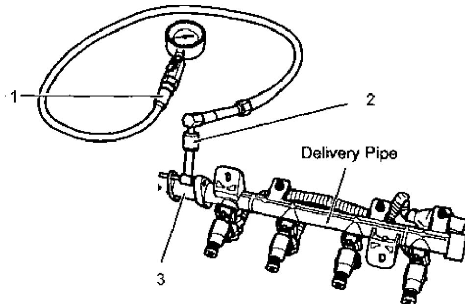
35-rasm. Yonilg'i ta'minot tizimidagi bosimni tekshirish: 1-manometr; 2-ulgich; 3-quvuro'tkazgich.
