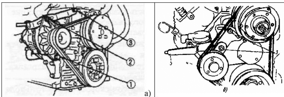
30-rasm. Dvigatellardagi yuritma moslamalarining tarangligini ostlash: a-Isuzu, b-ZMZ-53, v-ZIL-130 1-generator, 2- o'rnatish plankasi, 3-gayka, 4-taranglash roligi, 5-richag, 6-tirsakli val shkivi, 7-generator shkivi, 8- rostlash bolti, 9, 10, 11-kompresor, shamolparrak va suv nasosi, rul boshqarmasidagigidrokuchaytirgich nasosining shkiqlari, 12-taranglash kron-shteyni.
