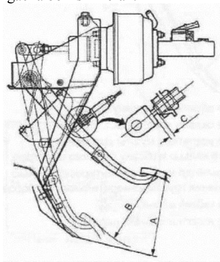
48- rasm. ISUZU avtomobilini ilashma muftasi tepkisini sozlash.
