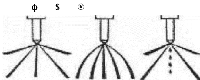
41-rasm. Forsunkaning yonilg'ini sepish holatlari: 1-me'yoriy; 2-nuqsonli (sepish teshiklari kirlangan); 3- nuqsonli (tomchilab sepilish).
