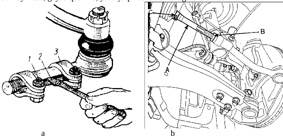
53-rasm. Klassik modeldagi (a) VAZ avtomobillarning yaqinlashuv burchak-larini sozlash. XUNDAI (b) avtomobilining yaqinlashuv burchagini sozlash.
