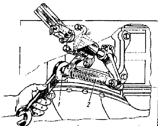
47-rasm. ZIL-130 avtomobilidagi mexanik yuritmalilashma tepkisining erkin yo'lini rostdlash 1 -tortqidagi gayka; 2-ajratish ayrisini tutashtirib turuvchi tortqi
