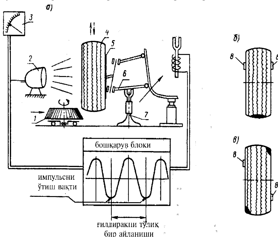
55-rasm. Harakatlanuvchi muvozanatlash jihozining ishlash shakli
