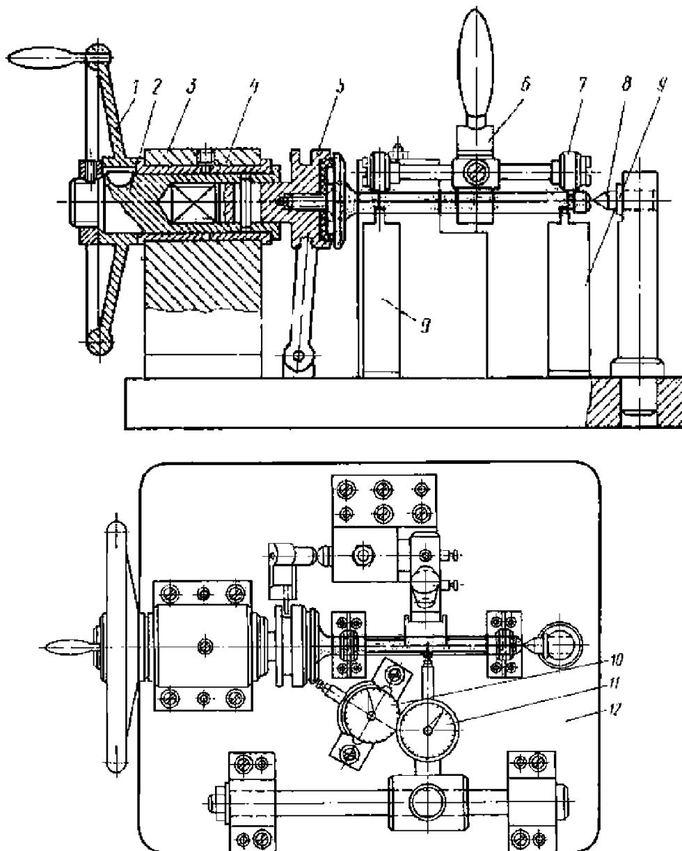
26-rasm. Klapanlarni tekshirish moslamasi: 1-maxovik; 2-valcha; 3-ustuncha; 4-vtulka; 5-barmoq; 6-kronshteyn; 7-rolik; 8-markaz; 9-prizma; 10, 11-indikatorlar; 12-plita
