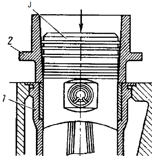
23-rasm. Porshen yig'masini tsilindrda o'rnatish: 1-tsilindr blokidagi gil'za; 2-moslama; 3-porshenning shatun va halqalar bilan birgalikdagi yig'masi
