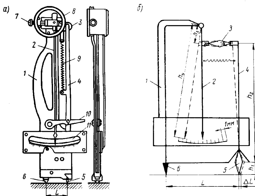
8.8-rasm. Tenzometr:
