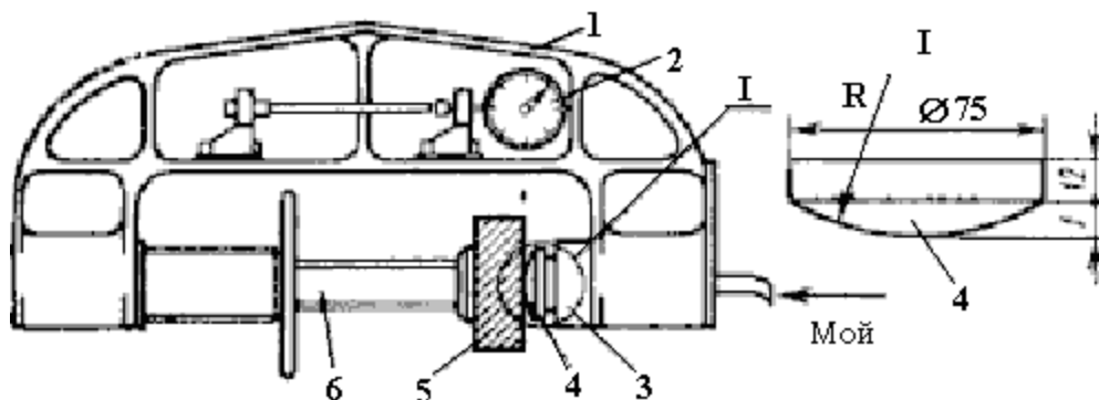
9.2-rasm NIIJB shtampi. 1-dinomometr strubtsinasi, 2-indikator, 3-gidravlik nasos, 4-shtamp, 5-sinalayotgan mahsulot, 6-sharnirli tayanch.
