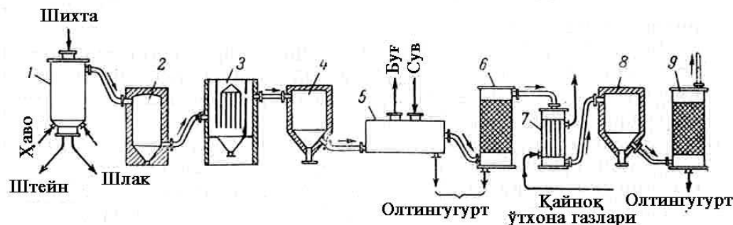
6.2 – rasm. Mis kolchedanidan oltingugurt bug‘i olish sxemasi:
