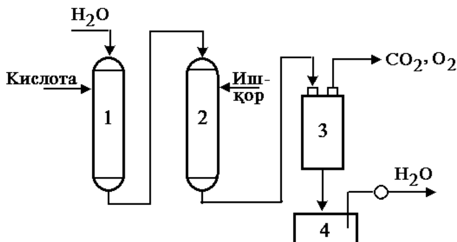
4.2 – rasm. Suvni yumshatish uchun qurilma sxemasi:
