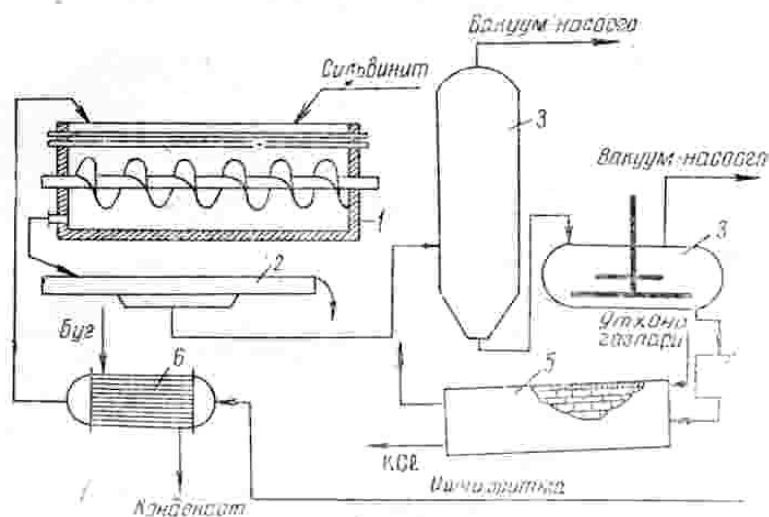
7.6 – rasm. Silvinitdan kaliy xlorid ishlab chikarishning prinsipial sxemasi.
