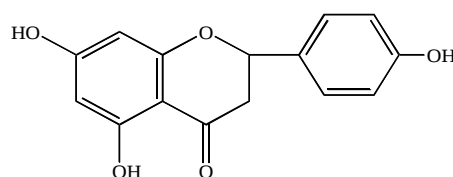
Naringenin
