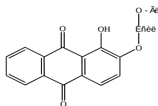
Ruberythric acid
