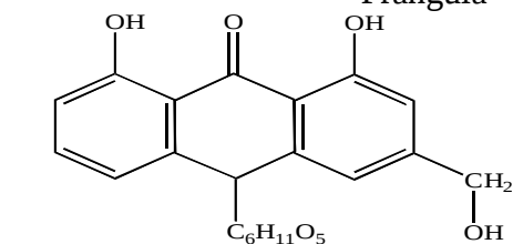
Aloe-emodin-anthrone glycoside
