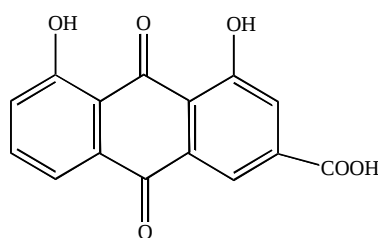
Rein
