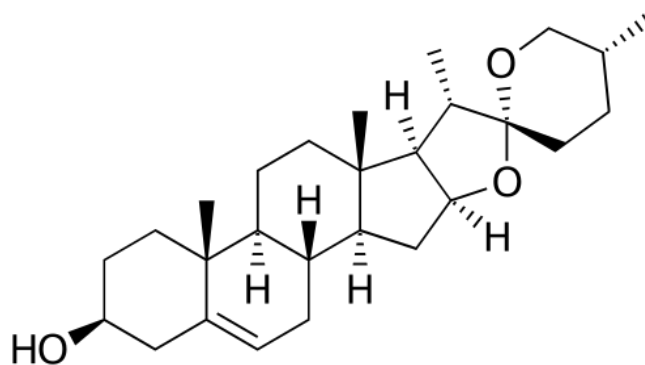
Diosgenin
