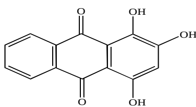
Purpurin
