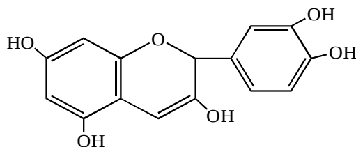
Tsianidin
