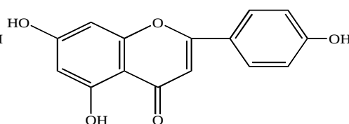
Apigenin
