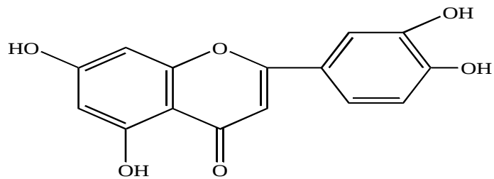
Luteolin
