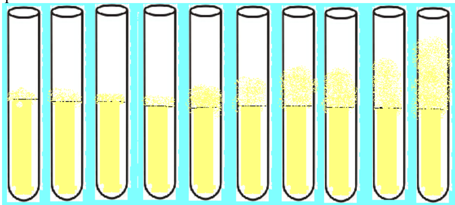
1.3.-rasm. Ko'pirish sonini aniqlash.
