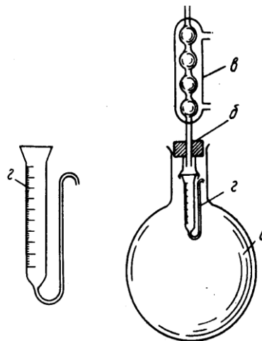
8.1-rasm.Ginzberg asbobchasi
