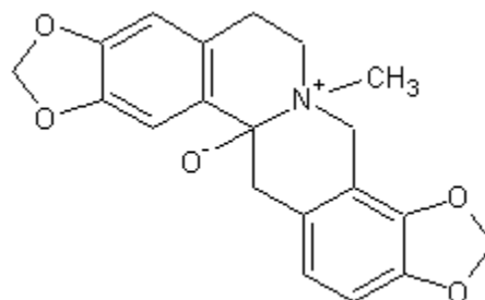
Protopin
