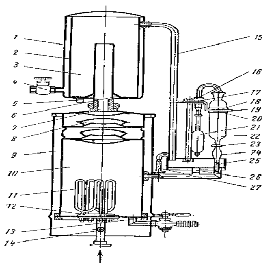
25-rasm Apyrogen suv olish apparati – AA - 1
