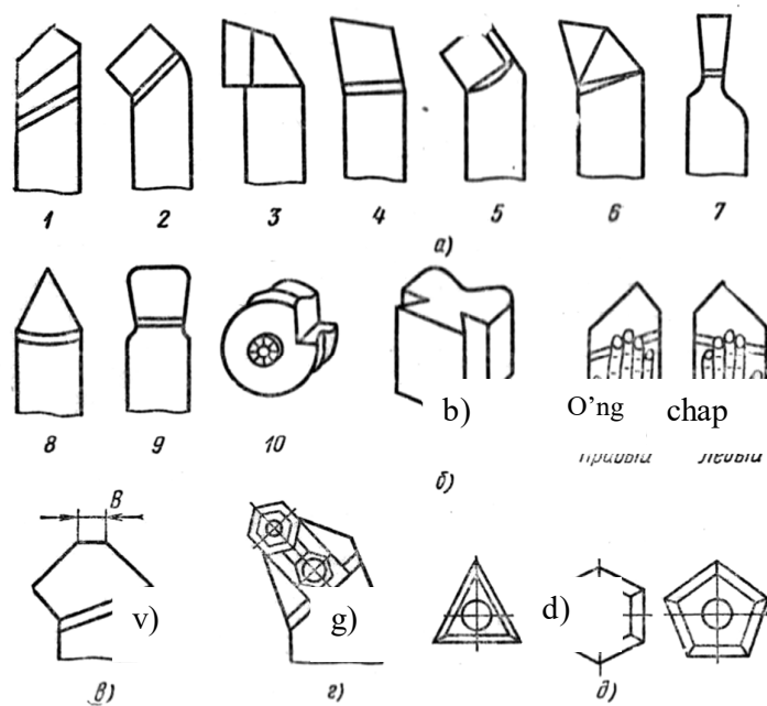
19.3-rasm. Tokarli keskichlar.
