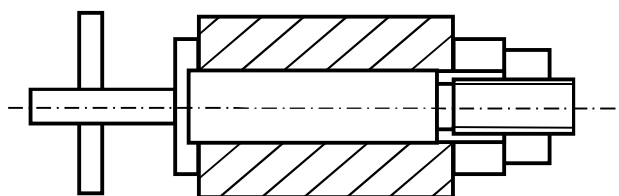
18.6-rasm. Ponasimon opravkaga o'rnatish.
