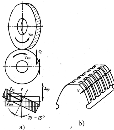
22.12-rasm Tishshevinglash sxemasi.
