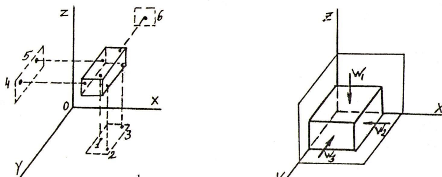
6.1 – rasm. Prizmatik detallarni asoslash
