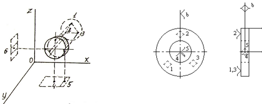
8.5 – rasm. Disk detallarni asoslash.
