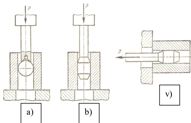
23.2-rasm. Teshik kalibrlash sxemalari.
