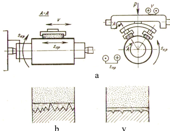
24.7-rasm. Superfinishlash usuli sxemasi.
