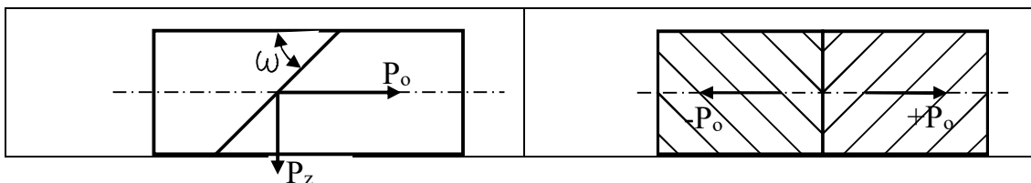
20.9- rasm. Oiva tishli frezalardagi kuchlar.
