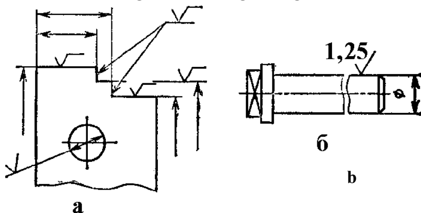
12.4-rasm. Yuza g'adir-budurligini belgilash misollari.
