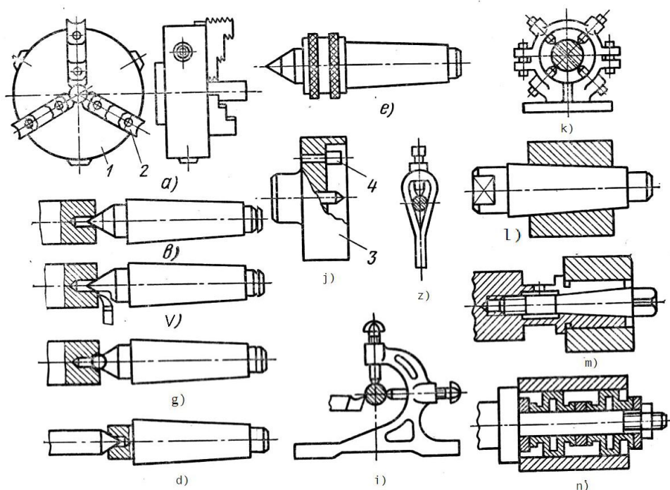
19.4-rasm. Tokarlashda ishlatiladigan moslamalar
