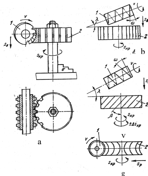
22.9-rasm. Tishfrezalash usuli.
