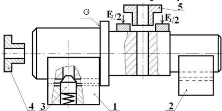
9.2-rasm. Detalni bazalashning nazariy sxemasi
