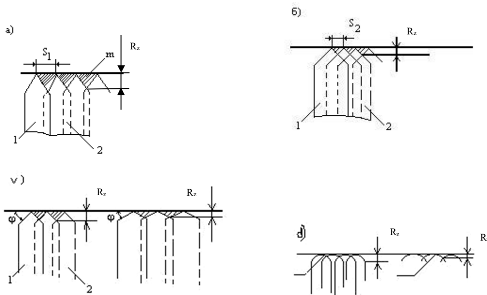
12.8 – rasm. G'adir-budurlik hosil bo'lishini geometrik sabablari.
