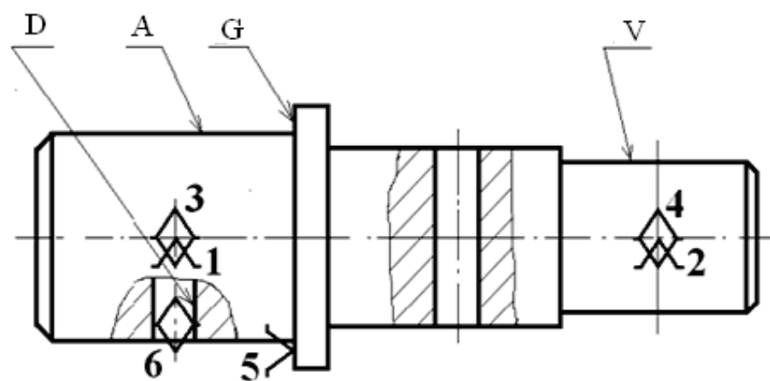
9.2-rasm. Detalni bazalashning nazariy sxemasi
