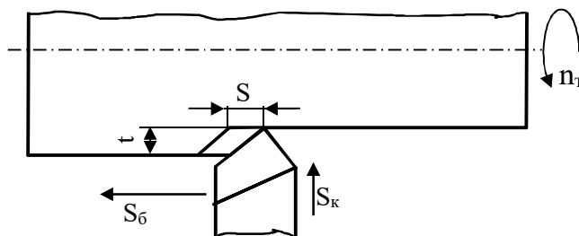
19.1 – rasm. Silindrik yuzaning tashqi sirtiga ishlov berish.
