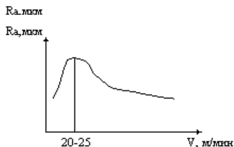
12.9-rasm. Kesish tezligini yuza g'adir-budurligiga ta'siri.
