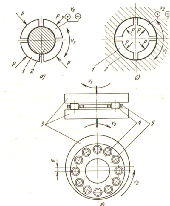
24.6-rasm. Artish sxemalari
