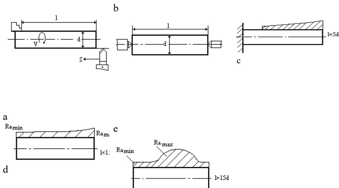
3.12 – rasm. DMAD tizimini g'adir-budurligiga ta'siri.
