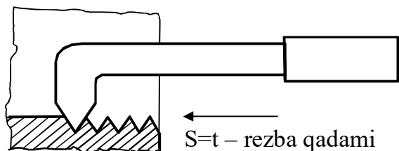
21.4- rasm. Keskichda rezba kesish jarayoni
