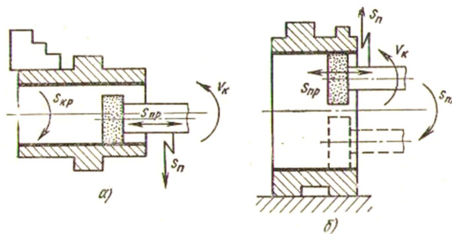
24.4-rasm. Doirali ichki jilvirlash sxemalari
