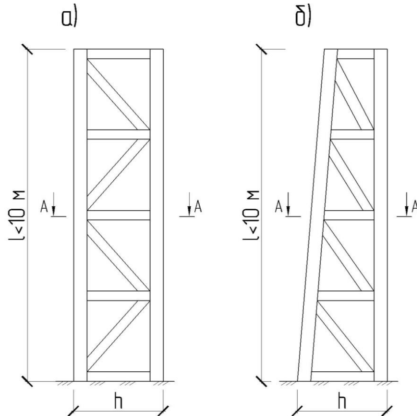
Figure 17 - Lattice props
