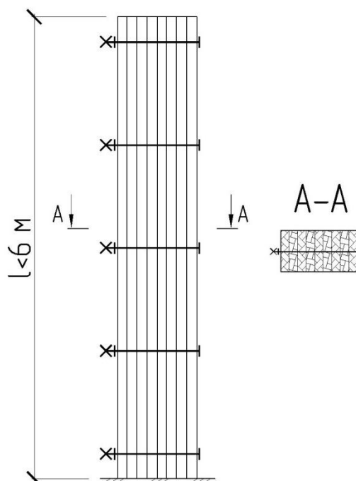
Figure 16 - Composite plank column
