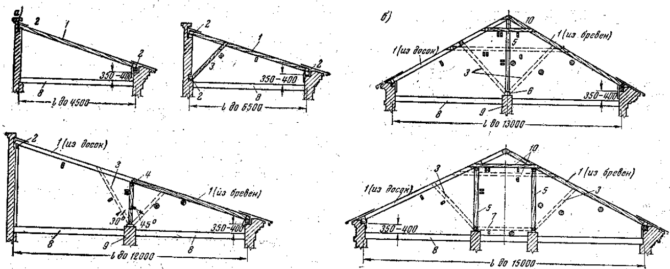
Figure 10. Inclined rafters:
