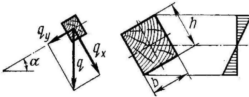
Figure 9. The oblique bend
