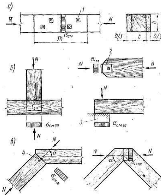
Figure 5 - Frontal stops:
