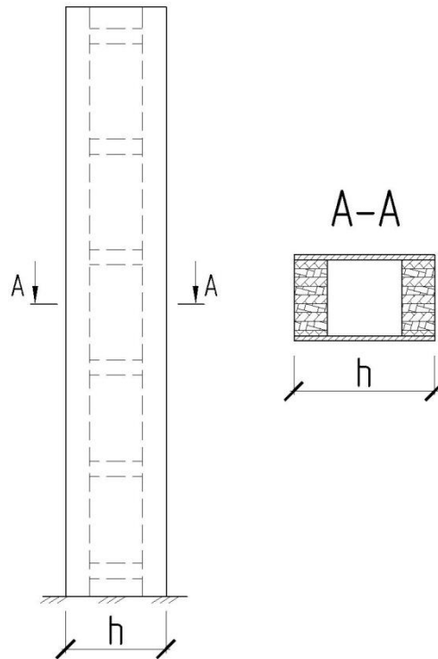
Figure 13 - Glue stakes
