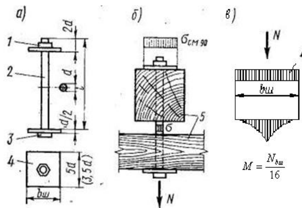
Figure 7 - Stretch bolts: a - general view; b - bolt and wood scheme; c - washer scheme; 1 - nut; 2 - rod; 3 - head; 4 - washer; 5 - elements to be connected
