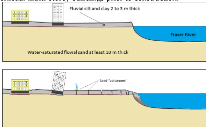
Figure 3.6 Recent unconsolidated sedimentary layers in the Fraser River delta area (top) and the potential consequences in the event of a damaging earthquake.
