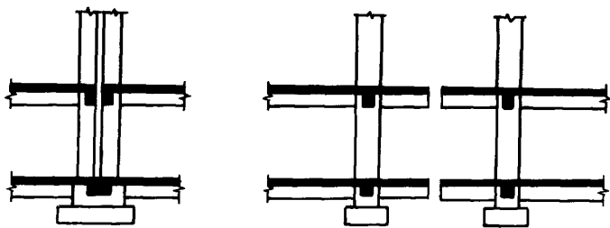
Figure 11.2. Anti-seismic joints in frame buildings
