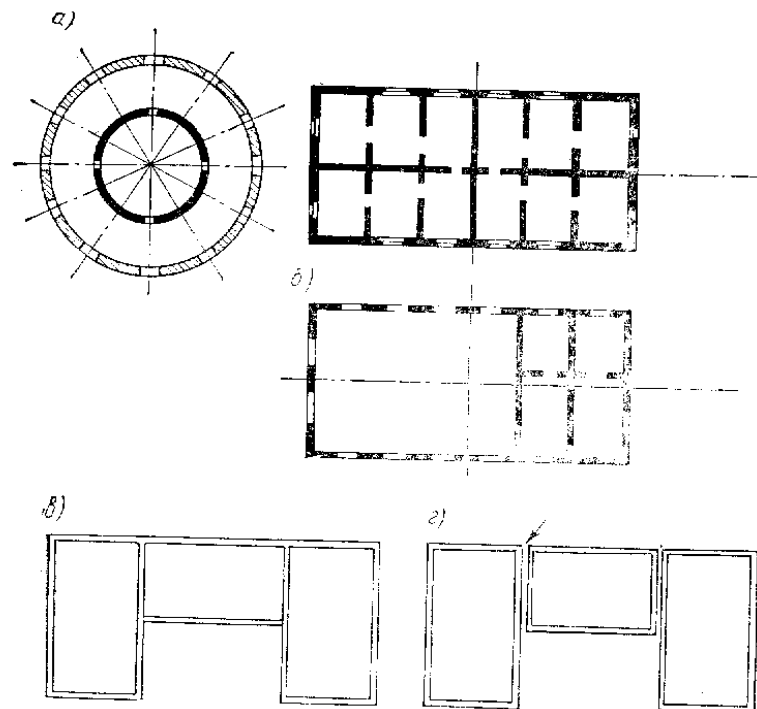
Figure 8.2. Seismic-resistant buildings plan: \alpha -symmetric building; b-symmetrical building; b, r,- complex shaped building (a-incorrect solution; r- correct solution)
