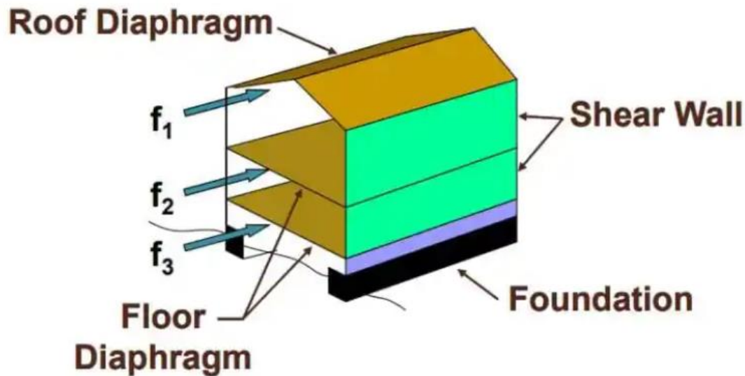
Fig. 3: Lateral Force Resisting System in a House
