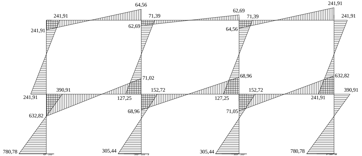
Figure 13.1. Regarding the first form of vibrations curve of bending moments.
