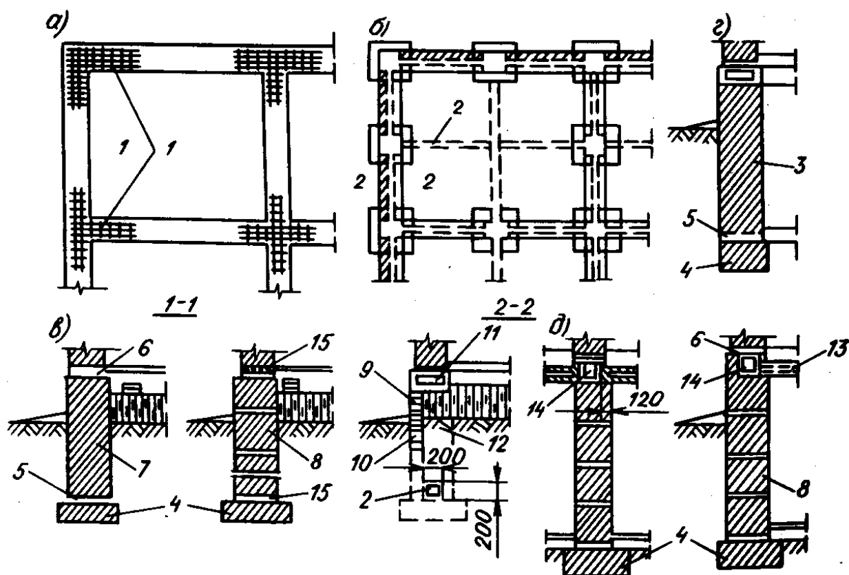
Figure 12.3. Details of the foundation and basement walls:
