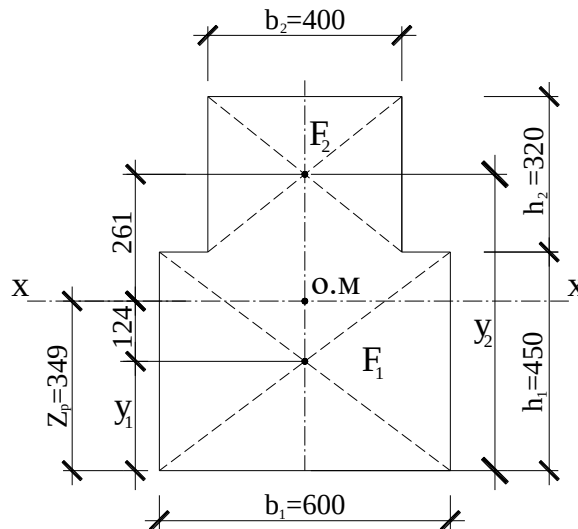
Figure 4.1. Cross-sectional surface of the Rigel.
