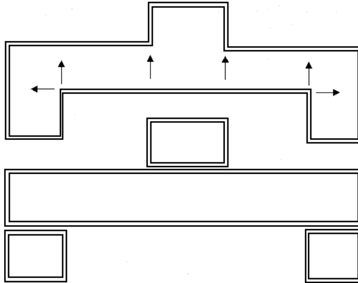
Fig. 8.3. Separation of complex-shaped buildings into simple-shaped parts according to earthquake resistance requirements. a- a solution that is not recommended when designing buildings in seismically active areas: b- division of the building into simple parts
