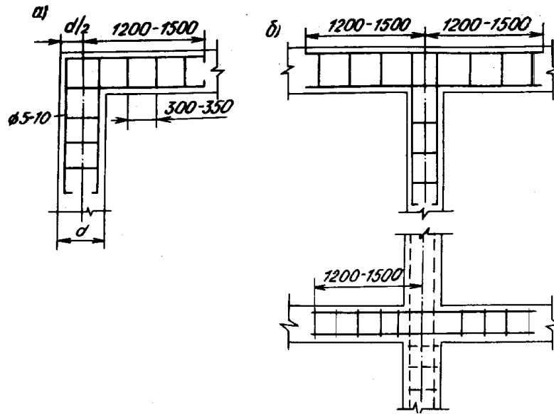
Figure 12.1. Joints of longitudinal and transverse walls: a) corners, b) intersections
