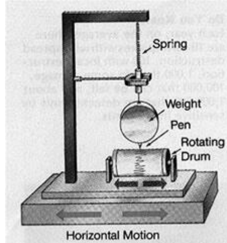
Figure 4.1. Sketch of a traditional seismometer. (Public domain.)
