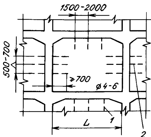
Figure 11.1. Attaching the wall to the frame: 1 – connections; 2 fittings
