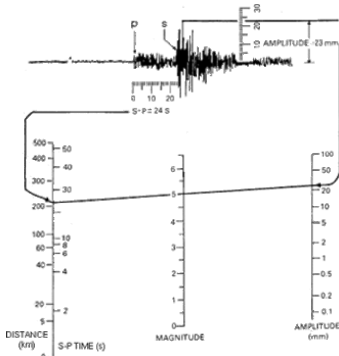
Figure 4.2. From Richter's (1958) book, Elementary Seismology . (Public domain.)
