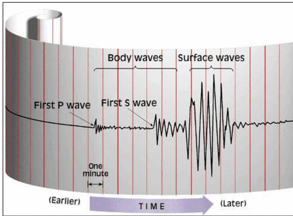
Figure 5.1. Body Waves and Surface Waves
