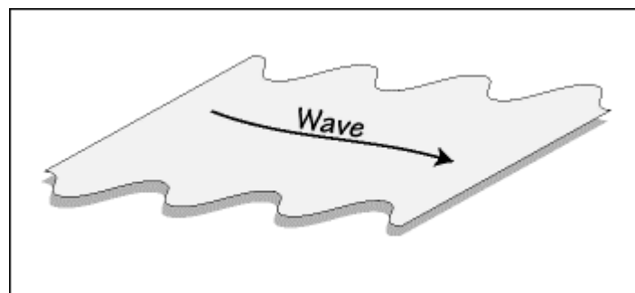
Figure 5.2. Love waves are transverse and restricted to horizontal movement
