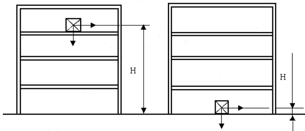
Figure 8.4. Reducing the seismic impact by placing the main technological processes and warehouses in the buildings on the first lower floor.
