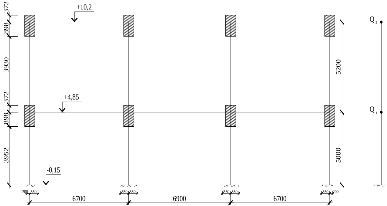
Figure 6.1. Calculation scheme of the transverse frame of the building frame.
