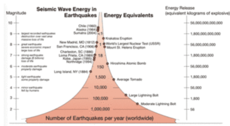
Figure 4.3. Earthquake magnitudes and energy release, and comparison with other natural and man-made events. (Courtesy Incorporated Research Institutes for Seismology, IRIS.)
