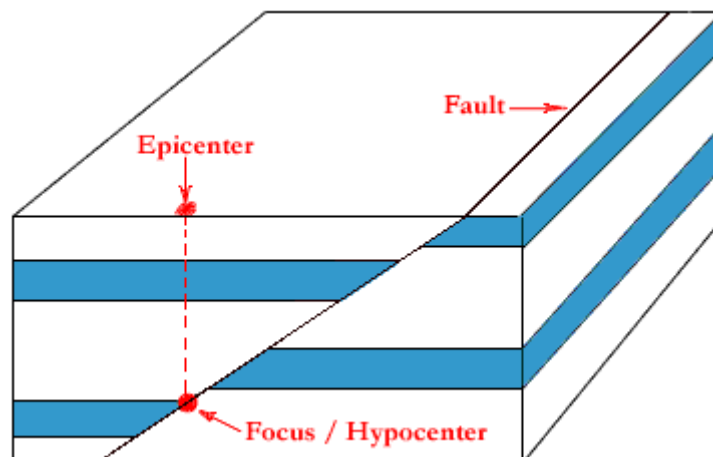
Figure 1. Diagram showing the relationship between the focus, or hypocenter, and the epicenter. The hypocenter is directly located on the fault plane, while the epicenter is the vertical projection of the hypocenter onto the ground surface.
