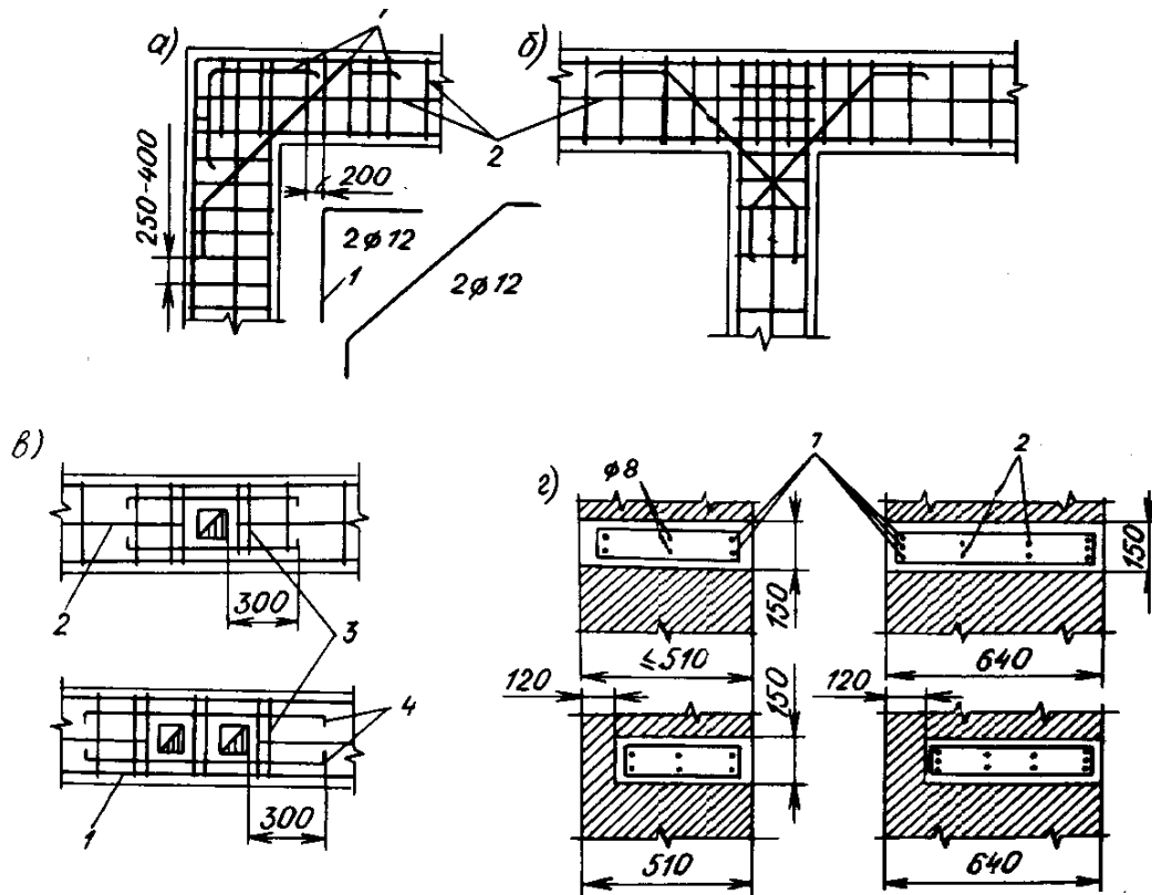
Figure 12.2. Details of anti-seismic belts:
