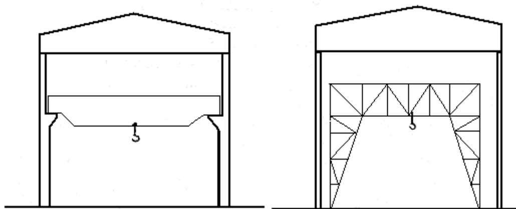
Figure 8.5. Reducing seismic impact by replacing overhead cranes with floor cranes.
