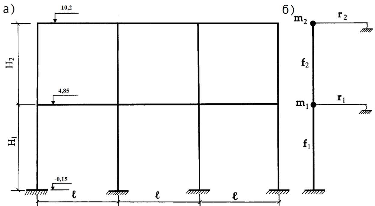
Figure 5.1. Static (a) and dynamic (b) calculation schemes of the building frame.
