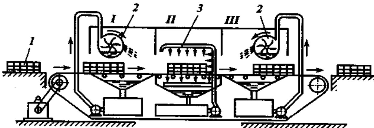
3.2-rasm. Detallardagi moyli ketkazish uchun uch kamerali yuvish mashinasining sxemasi
