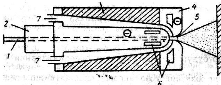
6.15-rasm. Plazma-yoy metallizatori kallagining sxemasi:
