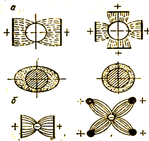
9.3-rasm. Anodlar (a) va ular shakllarining kuch chiziqdari harakteriga ta'siri (b)
