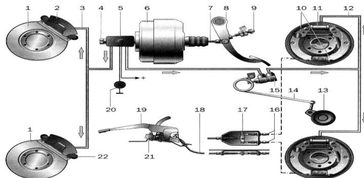
7.2-rasm. Avtomobil ishchi tormoz tizimining printsiptial sxemasi:
