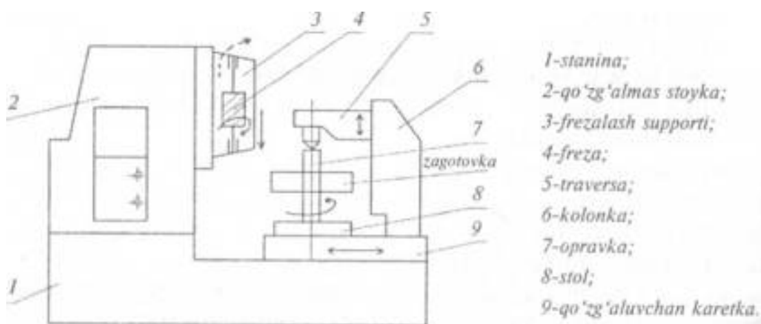
14.1-rasm. Tish frezalash stanogi.
