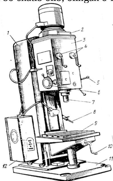
2-rasm. Rusumi 2A135 bulgan vertikal parmalash dastgoxi
