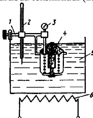
29-rasm. Termostatni tekshirish chizmasi: 1-kronshteyn, 2-termometr, 3-indikator, 4-termostat, 5-suvli vanna, 6-Elektir plitka
