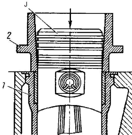
23-rasm. Porshen yig'masini tsilindrga o'rnatish: 1-tsilindr blokidagi gil'za; 2-moslama; 3-porshenning shatun va halqalar bilan birgalikdagi yig'masi
