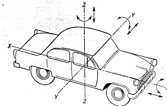
26.3-rasm. Avtomobilning tebranishi
