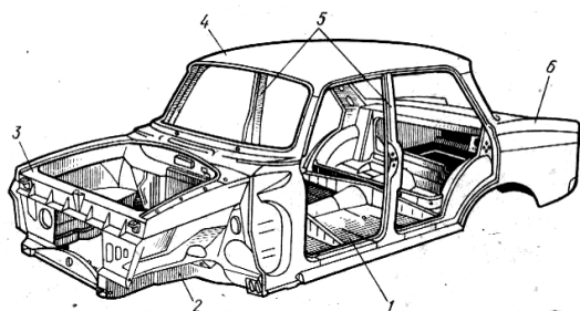
15.3-rasm. Yengil avtomobil kuzovining karkasi. 1-tag qism, 2-rama, 3-oldingi qism, 4-tom, 5-ustunlar, 6-orqa qismi
