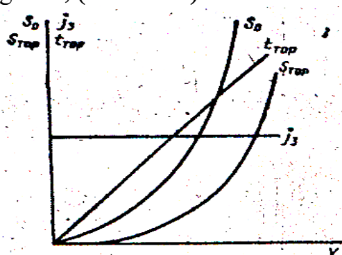
22.2-Rasm. Tormozlanish o'lchovlarining o'zgarishi
