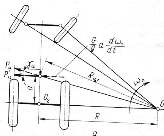
24.2-rasm. SHinalarning yonaki sirpanishi bo'lmaganda avtomobilning burilishi.
