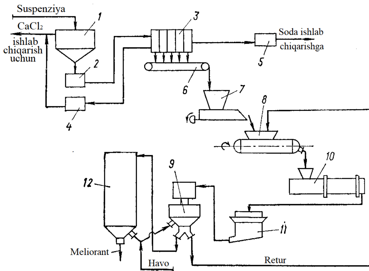
13.1-rasm. Meliorant ishlab chiqarish sxemasi: 1–tindirgich; 2 – oraliq sig'im; 3 – kamerali filtr-press; 4 – filtrat yig'itgich; 5 – yuvuvchi suvlarni yig'gich; 6 – transporter; 7 – bunker vibrodosator; 8 – aralashtiruvchi; 9 – pevm qurilma; 10 – barabanli quritgich; 11 – chukkishli maydalagich; 12 – silos.
