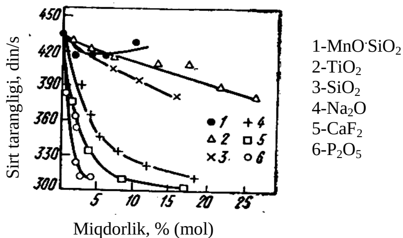
8.6-rasm. 27% CaO, 36% FeO, 6% Fe 2 O 3 , 31% SiO 2 tarkibli shlakka 1350°C da birikmalarning sirt tarangligiga ta'siri.
