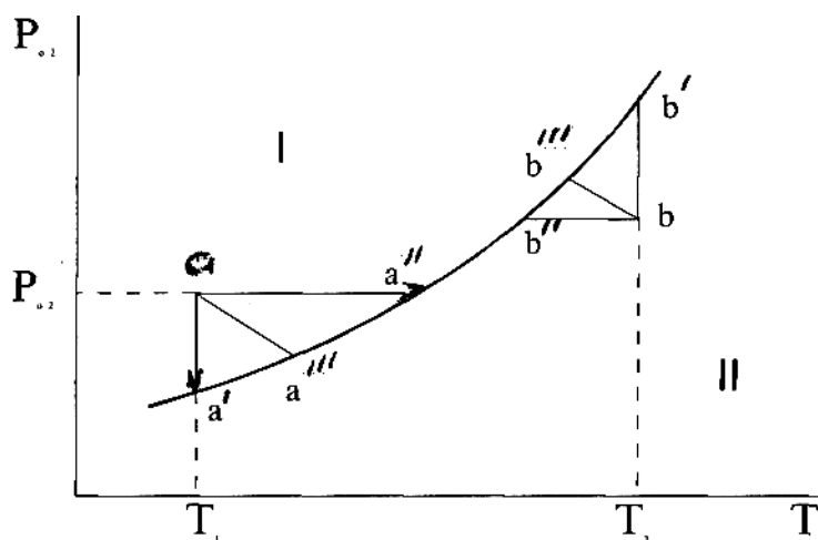
2.1-rasm. Ajralish jarayonida P_{O_2} ni haroratga bog'liqligi.
