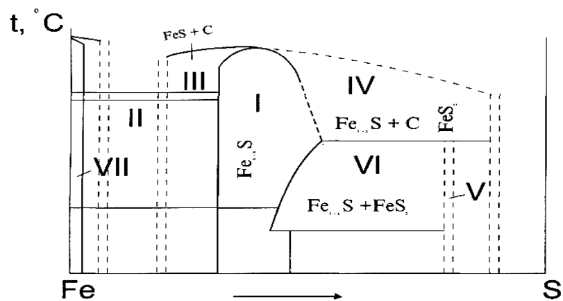
2.1-rasm. Fe-S sistemaning diagrammasi.
