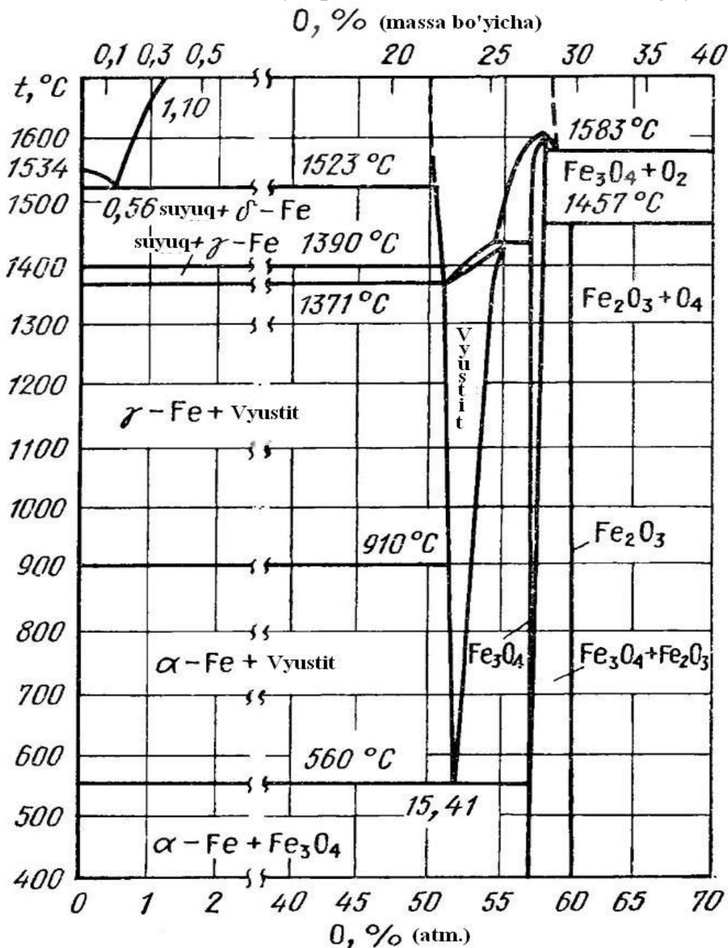
2.4-rasm. Fe – O sistemasining holat diagrammasi.
