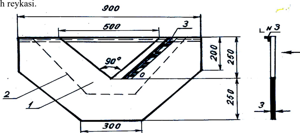
19-rasm. CHipoletti suv ulchash asbobi (CHSA-0,50).
