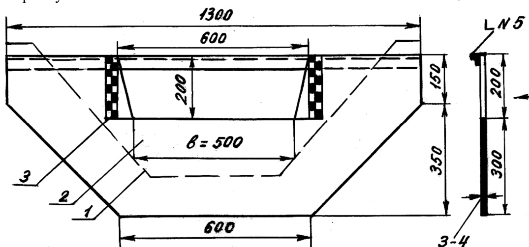
19-rasm. CHipoletti suv ulchash asbobi (CHSA-0,50).
