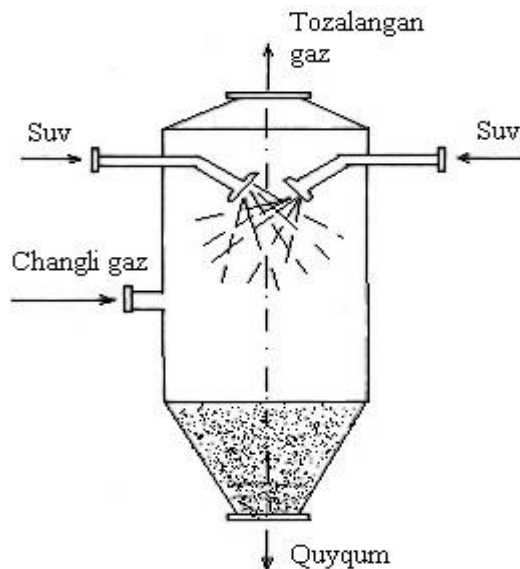
7-rasm. Forsunkali scrubber.
