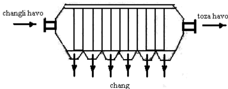
4-rasm. Sim pardali chang cho'ktirish kamerasi.
