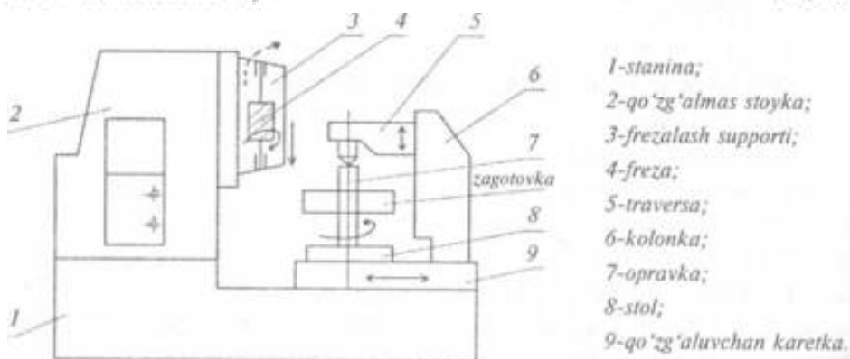
14.1-rasm. Tish frezalash stanogi.
