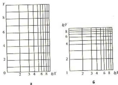
12.2-rasm. Yarim logarifmik (a) va logarifmik (b) koordinata to'rlari
