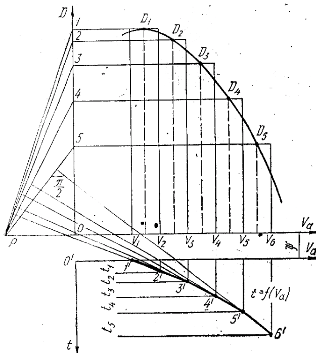
21.7-rasm. Tezlanish vaqtini grafik usulda aniqlash.
