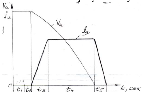
22.3-rasm. Avtomobilning tormozlanish grafigi
