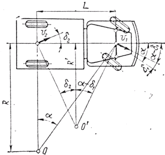
24.1-rasm. SHinalarning yonaki sirpanishi bo'lmaganda avtomobilning burilishi.
