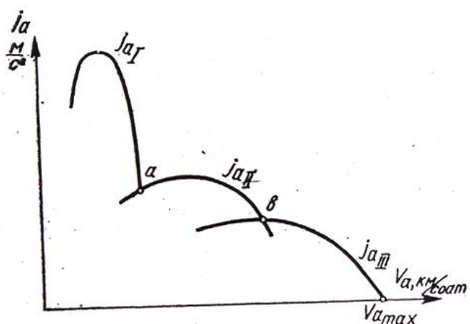
21.3-rasm. Avtomobillarning tezlanish tavsifi
