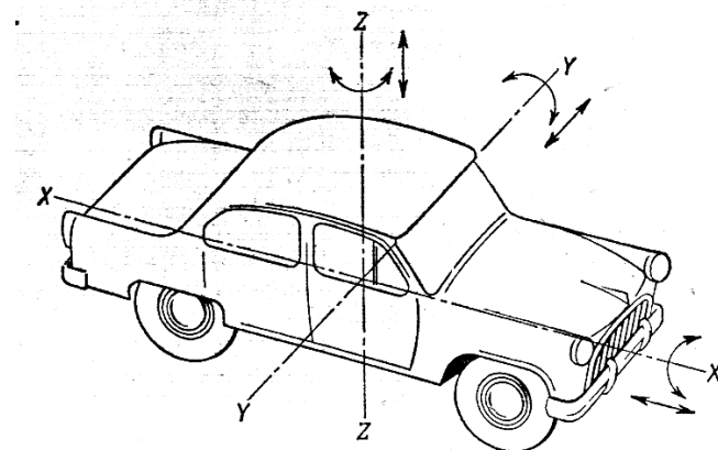
26.3-rasm. Avtomobilning tebranishi
