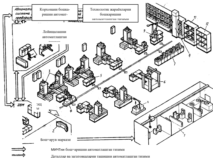
3.3-rasm. Moslanuvchan ishlab chiqarish tizimi
