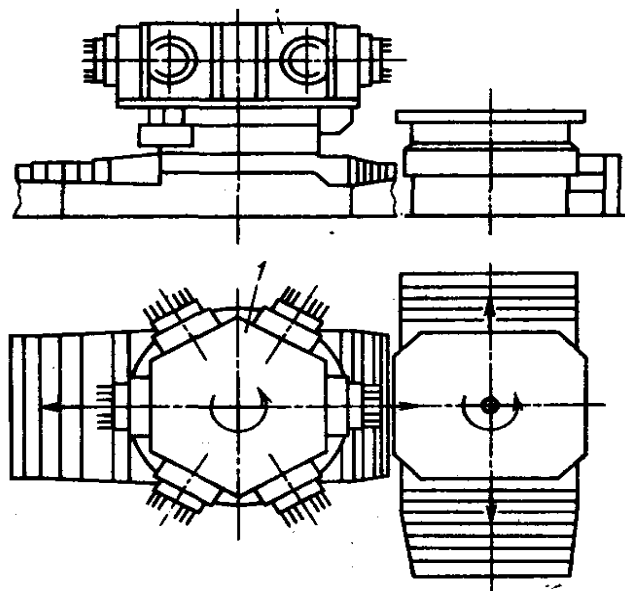
3.2-rasm. Revolver kallakli agregat dastgoh sxemasi
