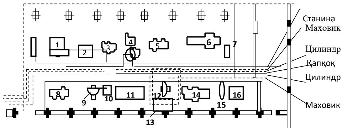
7.1-rasm. Mexanika tsexida detallar harakatining sxemasi
