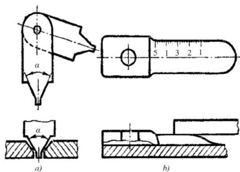
1.1-rasm. Payvand birikmalarni yig'ishni tekshirish uchun
