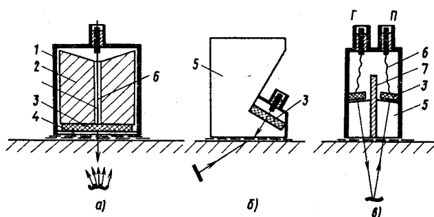
3.7 - rasm. Ultratovushli o'zgartkichlar:
