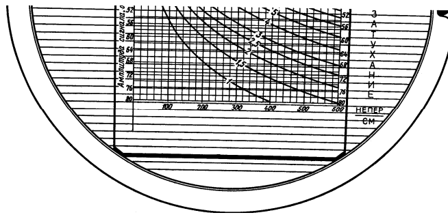
3.9-rasm. Pleksiglasli qiya izlagich uchun ARD-diagrammali planshet ( \alpha = 40^\circ , spezoplastinaning diametri 12 mm, f=2,5 Mgts):
