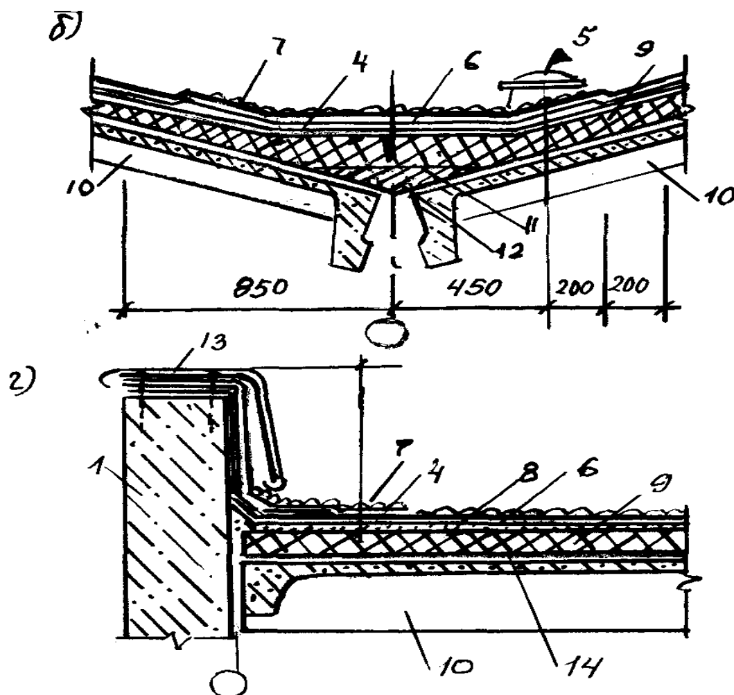
Rasm 29. Rulon tom yopma detallari
