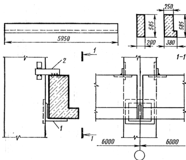
7.8-rasm. Ulama (bog'lovchi) to'sin va uning kolonkaga mahkamlanishi. a-po'lat taxta (list) tayanch; 2-po'lat planka; 3-payvod choki;
