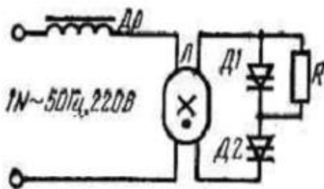
5-rasm. Lyuminescent lampani dinistor orqali ulash sxemasi.
