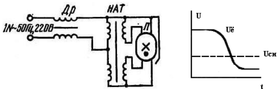
6-rasm. Lyuminescent lampni issiq yoquvchi ITA bilan ulash sxemasi (a) va yonish diagrammasi (b).
