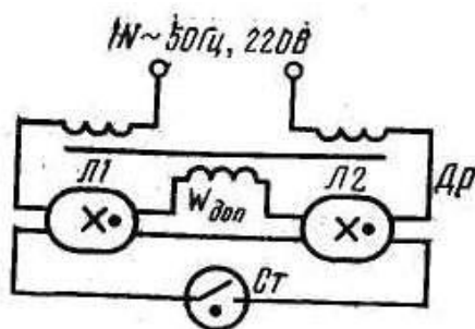
4-rasm. Lyuminescent lampalarini ketma-ket ulash sxemasi.
