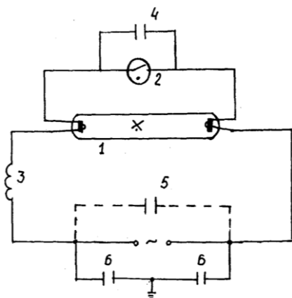
Rasm. Lyuminestsent chirog'ining ulanishi sxemasi
