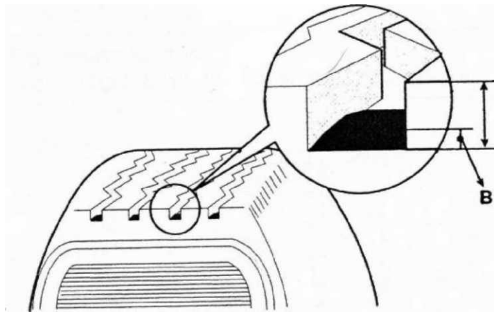
54-rasm. SHina rasmining yoyilish indikatori
