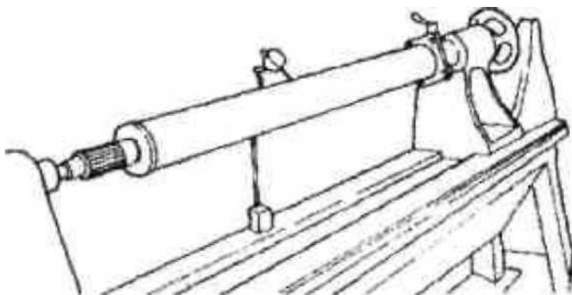
50-rasm. Kardan valini o'q bo'yicha urishini tekshirish.
