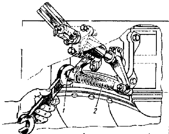
47-rasm. ZIL-130 avtomobilidagi mexanik yuritmalilashma tepkisining erkin yo'lini rostlash 1 -tortqidagi gayka; 2-ajratish ayrisini tutashtirib turuvchi tortqi
