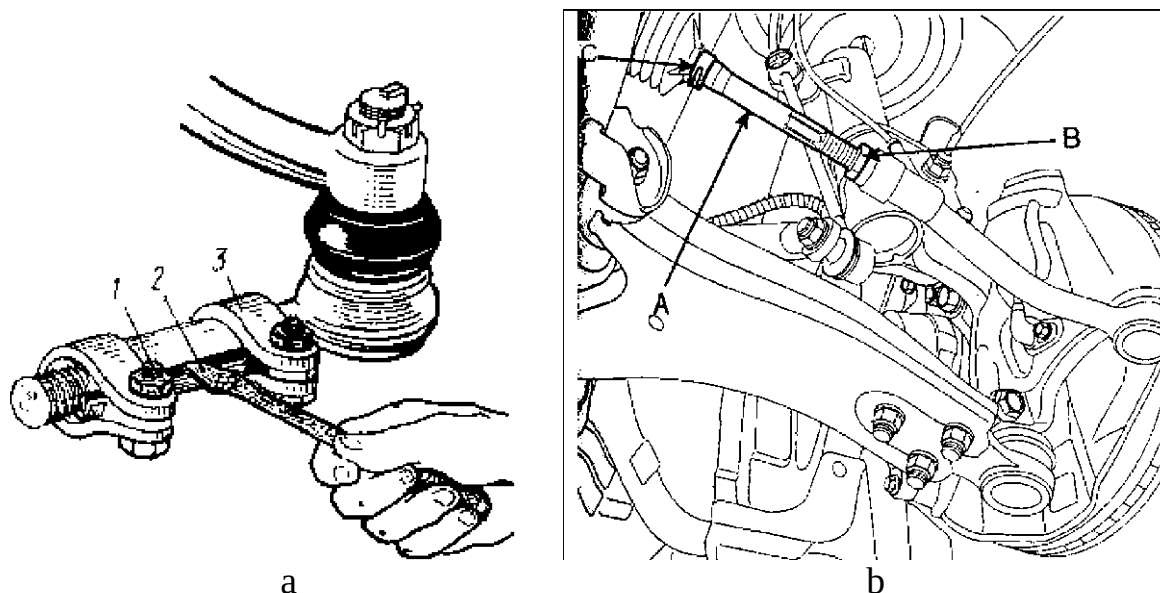
53-rasm. Klassik modeldagi (a) VAZ avtomobillarning yaqinlashuv burchak-larini sozlash. XUNDAI (b) avtomobilining yaqinlashuv burchagini sozlash.
