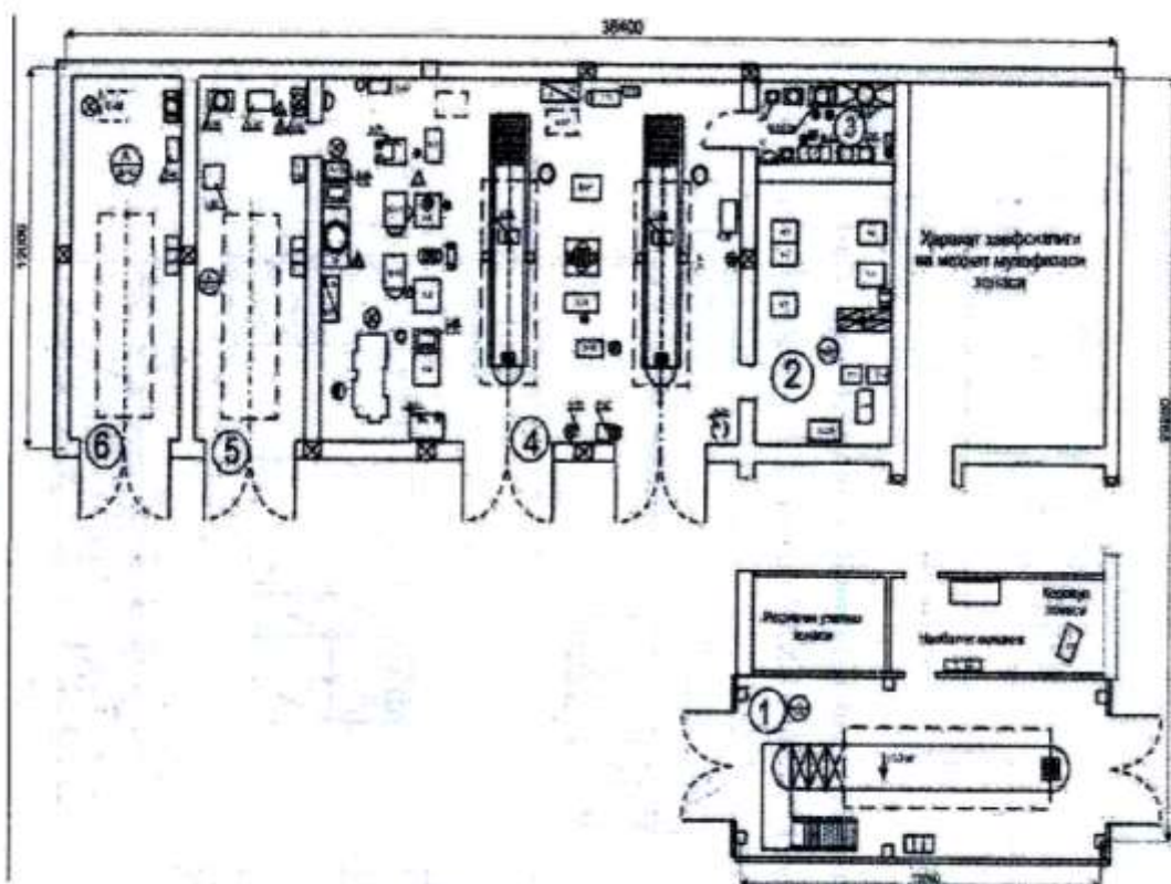
2.51-rasm. "Ozneftmahsulot" AK ga qarashli "Lrganchneftbaza" avtokorxonasining ishiab chiqarish binosi:
