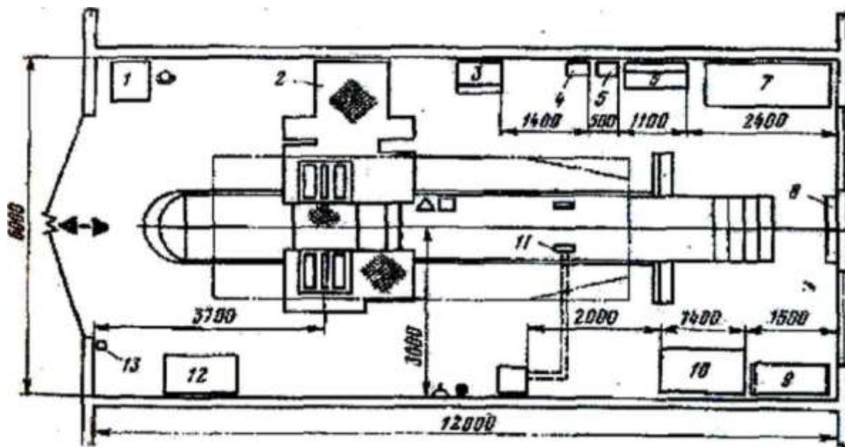
2.9-rasm. Yuk avtomobillari TSh-2 tashxislash mintaqasi rejasi:
