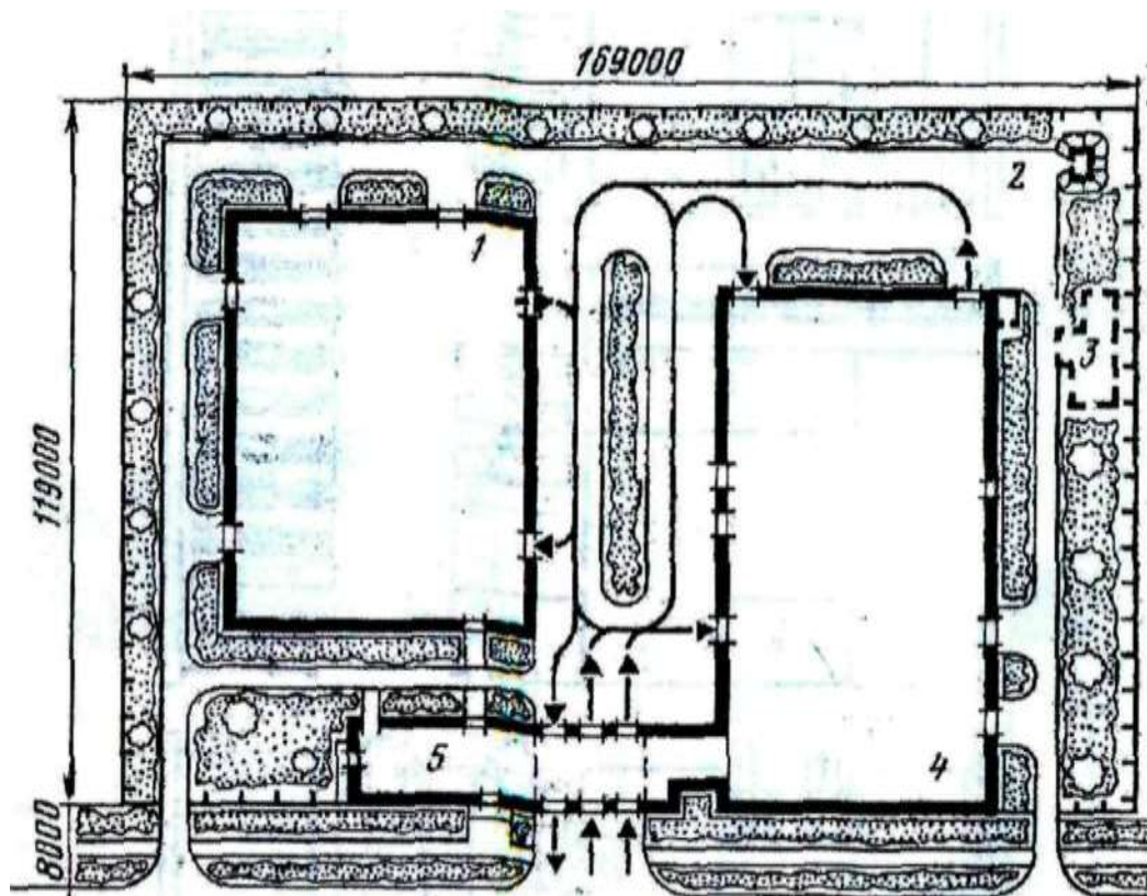
2.47-rasm. 650 ta avtomobil uchun taksomotor saroyining bosh rejasi:
