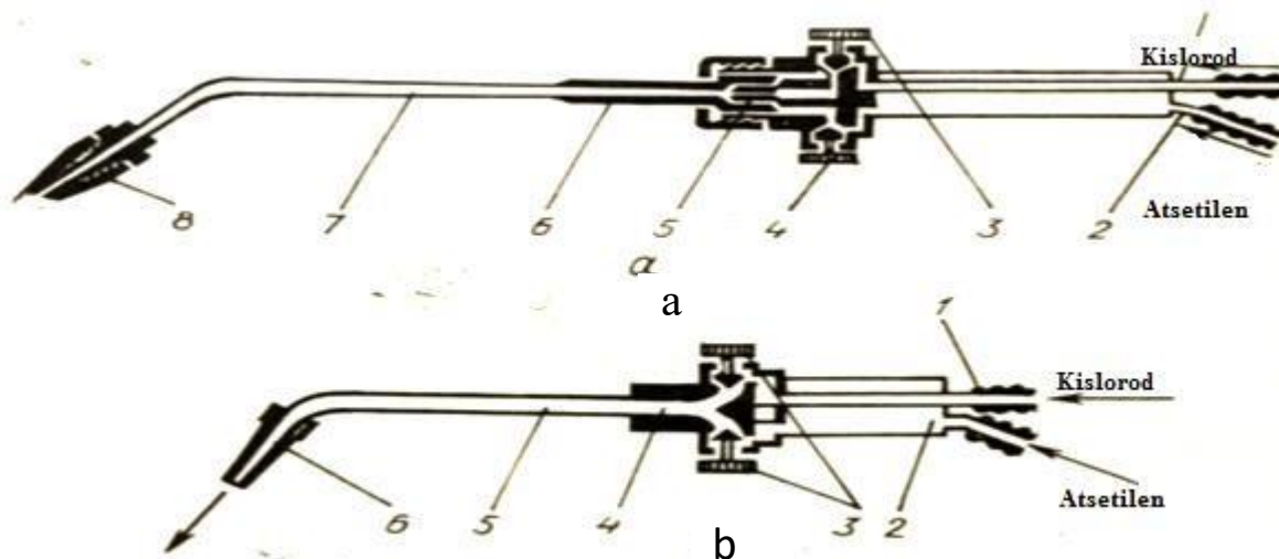
8.5-rasm. Payvandlash gorelkalari.
