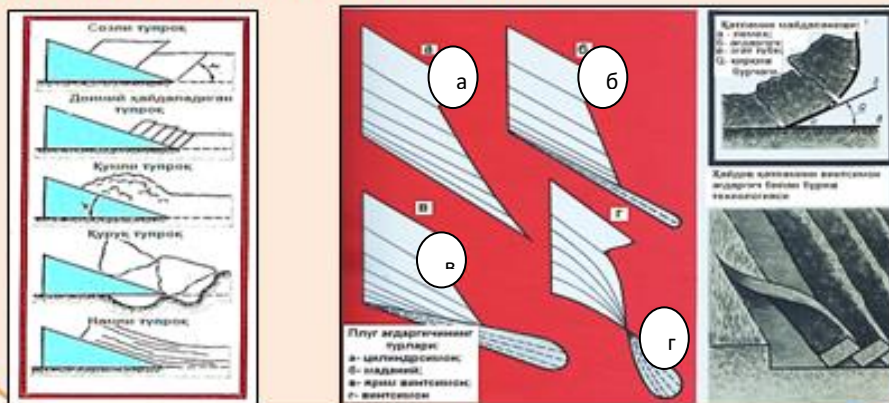
1.10-rasm. a-silindrik otvalli; b-madaniy; v-yarim vintsimon; g-vintsimon.
